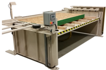
8100 Panel Feeder
