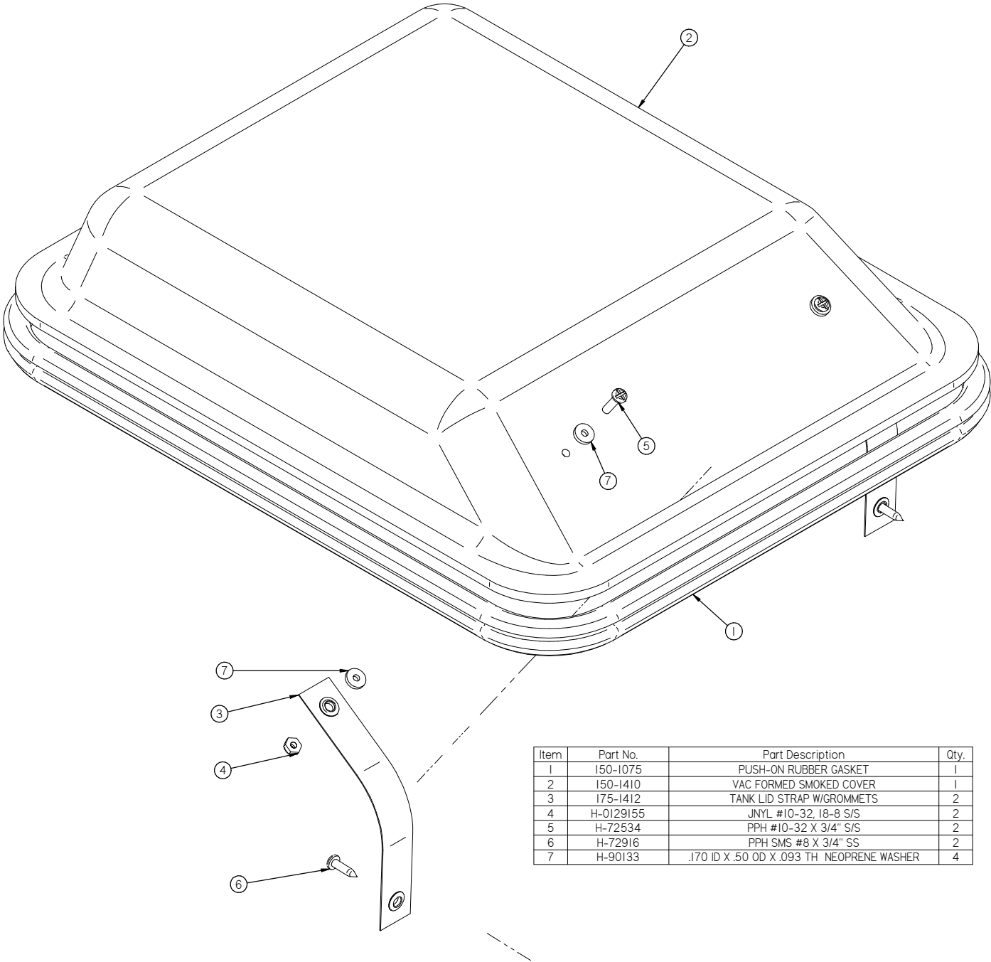
TANK LID ASSEMBLY 150-1410D
