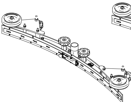
33 INCH SQUEEGEE ASSEMBLY 233-7180
