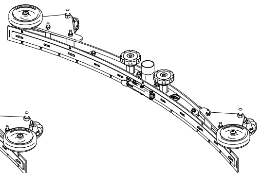
37 INCH SQUEEGEE ASSEMBLY 237-7180
