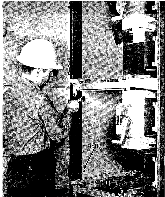
Fig. 49. Loosening of bolt holding side barriers in three-high enclosure.
