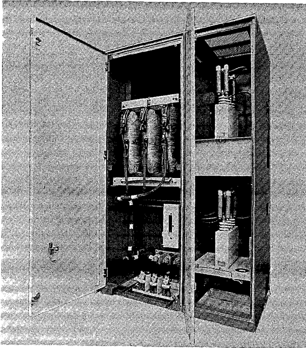
Fig. 16. Limitamp auxiliary enclosures for housing motor-starting reactors and power-factor-correction capacitors. Doors are mechanically interlocked or key interlocked.
