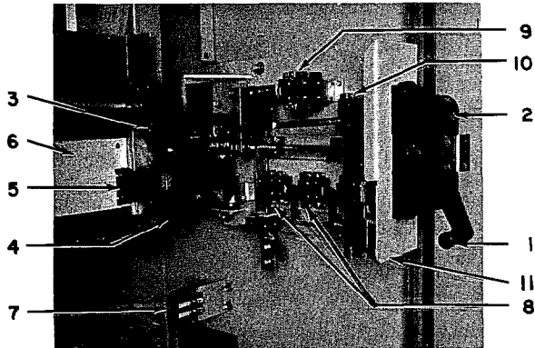
Fig. 96. Isolating switch, electrical interlocks and shutter mechanism in one-high enclosure.
