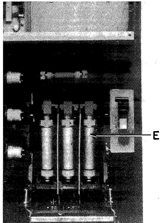
Fig. 83. Control-power transformers and fuses in one-high enclosures.
