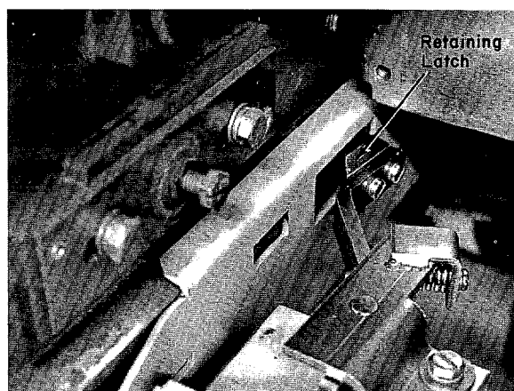
Fig. 46. Closeup of contactor, showing retainer latch.
