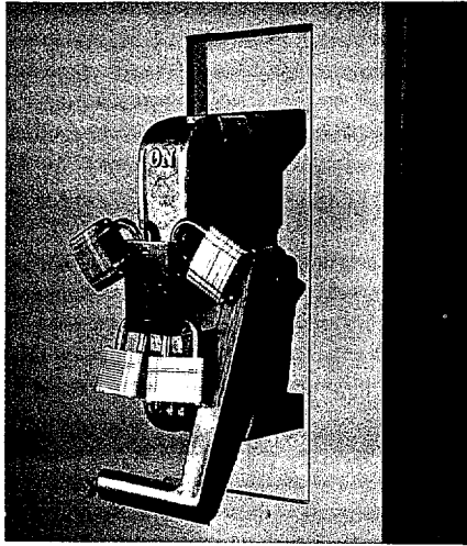
Fig. 8. Limitamp isolator handle padlocking provisions.
