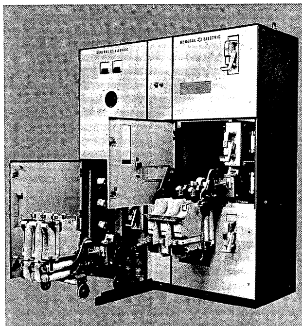
Fig. 91. One-high and three-high contactors in service position.
