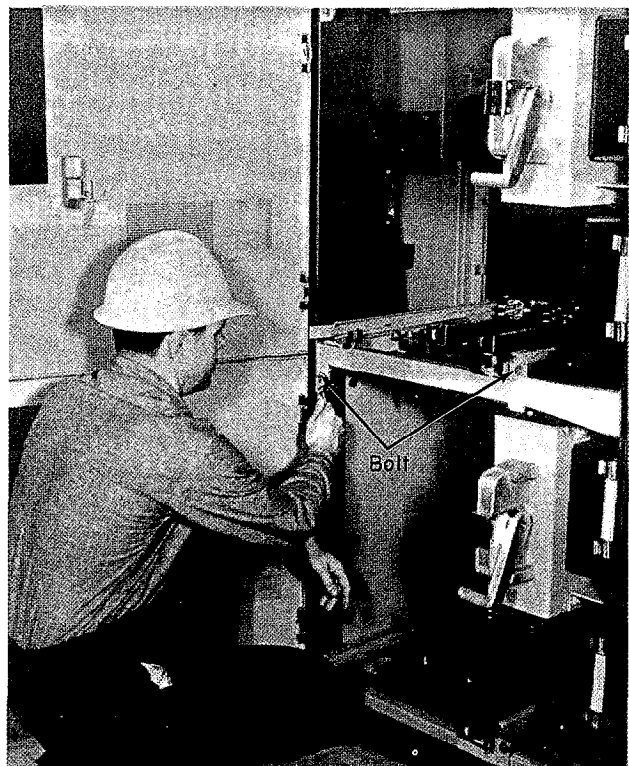
Fig. 50. Removing bolts in track and horizontal barrier assembly in three-high enclosure.
