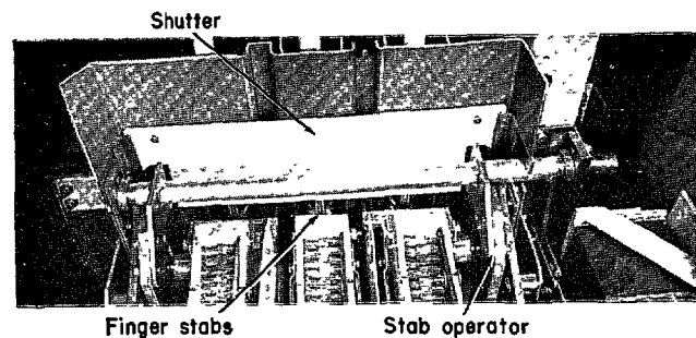
Fig. 13. Limitamp controller manually operated disconnecting stabs and shutter.
