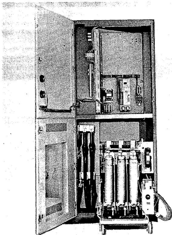
Fig. 9. 42-inch-wide enclosure with 630-ampere power fuses mounted on contactor.
