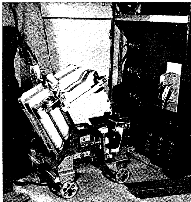
Fig. 92. Swinging high-voltage contactors open for inspection.
