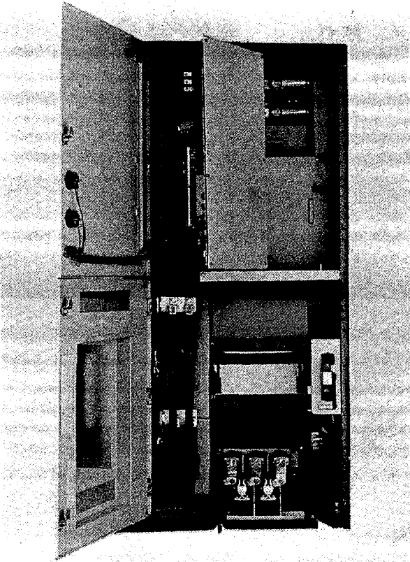
Fig. 67. Motor cable terminations in 42-inch-wide one-high enclosures.
