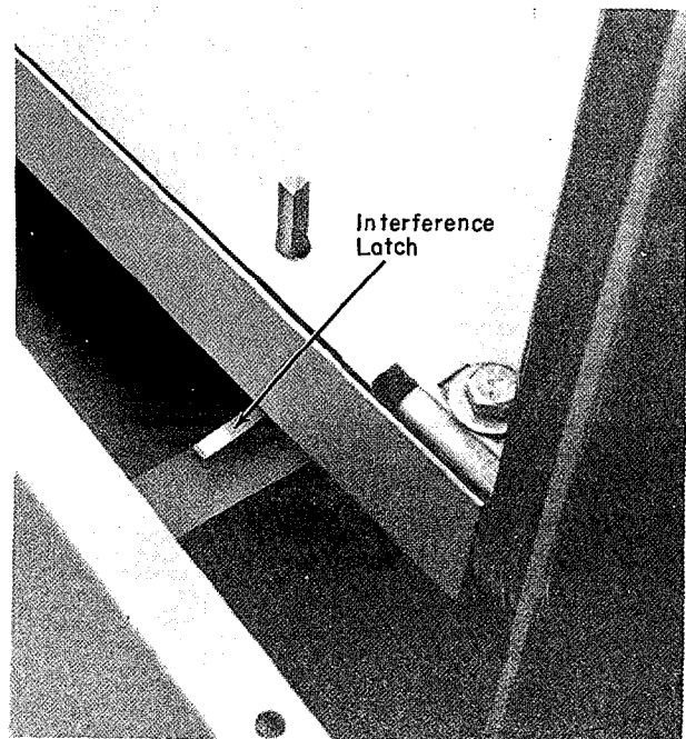
Fig. 87. Interference latch.
