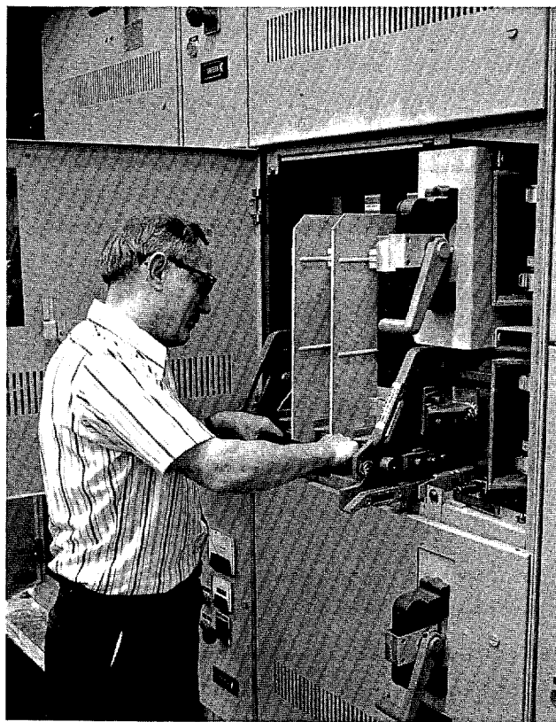
Fig. 45. Pulling on contactor positioning handle.
