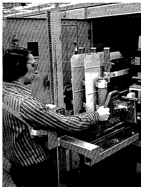
Fig. 36. Removing contactor, using Cat. No. 116C9918G1 lift.
