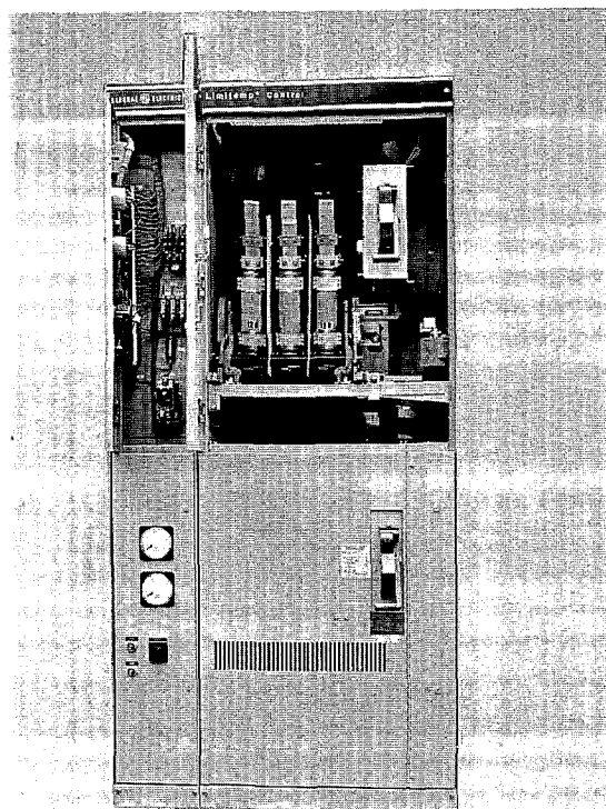
Fig. 32. Two-high enclosure with top high-voltage door open.
