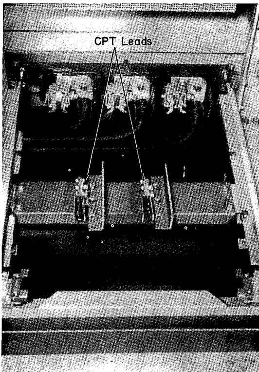
Fig. 48. Leads from the control power stabs.
