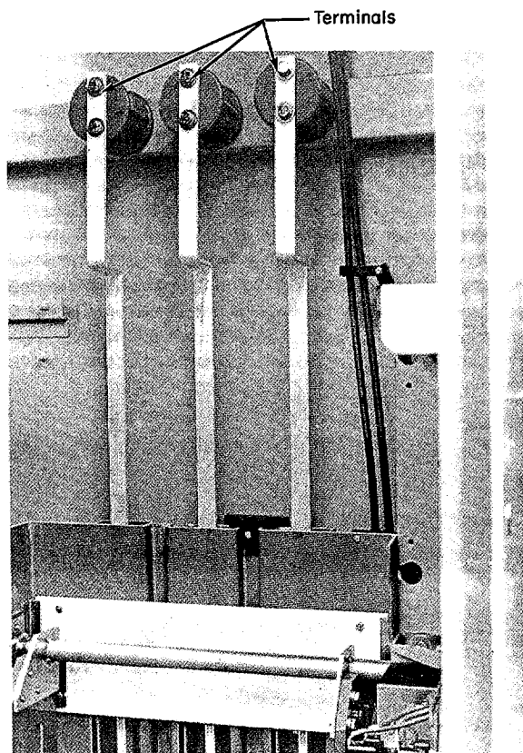
Fig. 57. One-high enclosure without horizontal bus showing terminal points at end of vertical bus.
