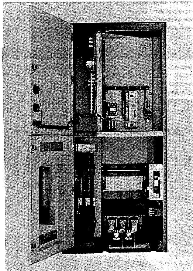
Fig. 75. 750-mcm cable terminated with Termi-Matic stress cones. For complete information refer to Bulletin IMF-126C.
