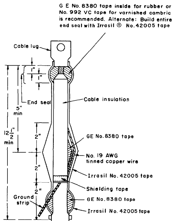
Fig. 73. Termination of shielded, 5000-volt cable showing stress-cone construction.
