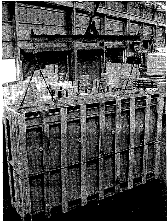
Fig. 20. Recommended method of lifting a Limitamp lineup. Note that the lineup is suspended from an equalizing bar.
