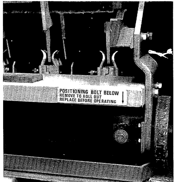
Fig. 25. One-high contactor in enclosure showing positioning bolt that must be removed to roll out contactor.
