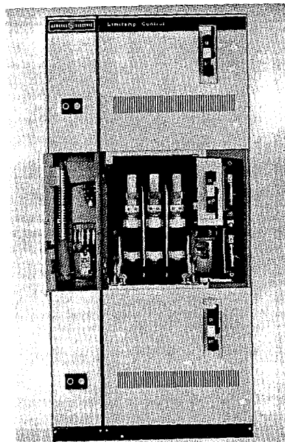
Fig. 7. Three-high design for compartment separation.
