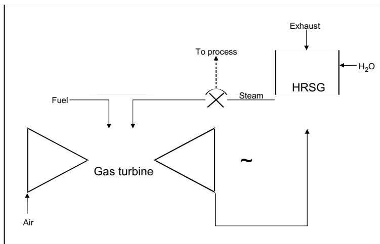
Figure 15. Typical STIG™ cycle
