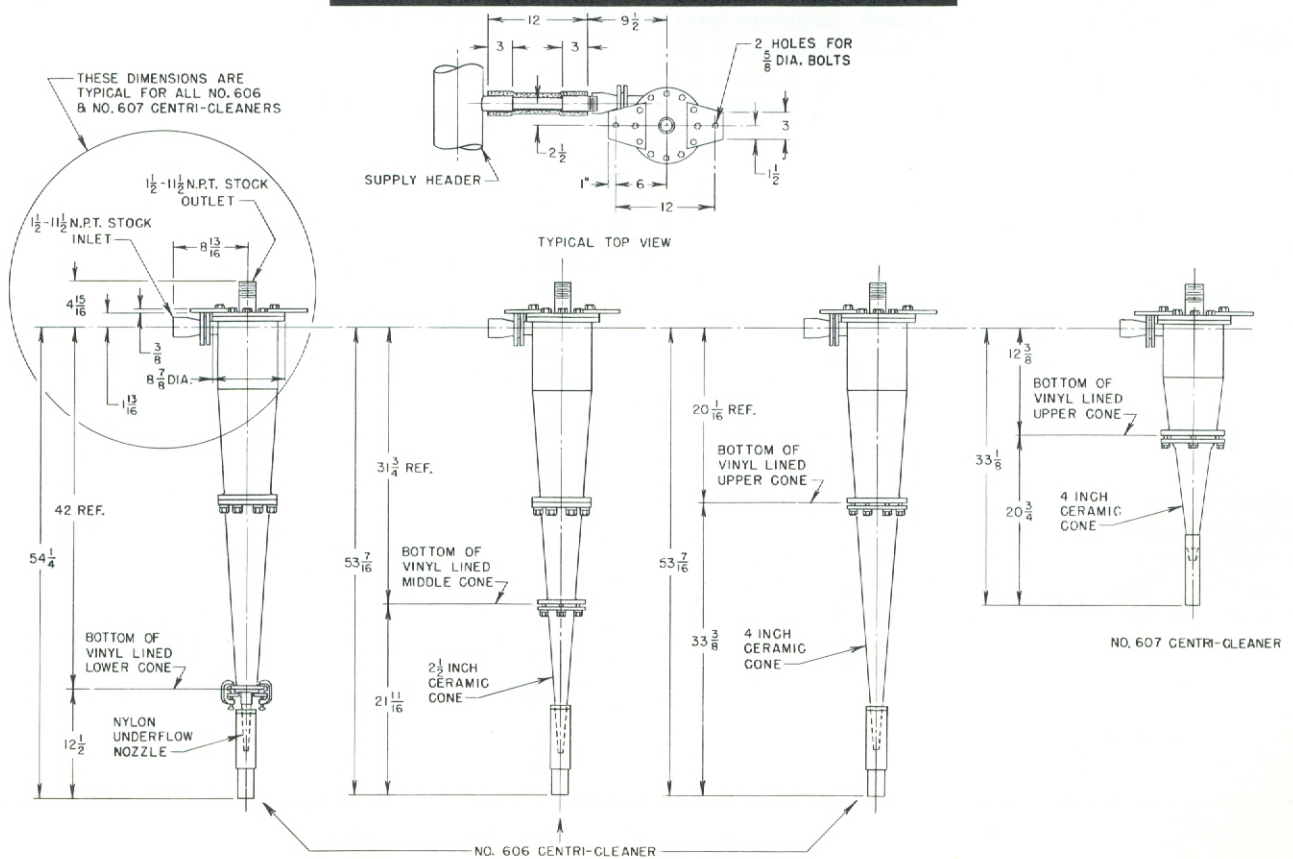
FIGURE 13: Dimensions of Bauer Cleaner Units.
