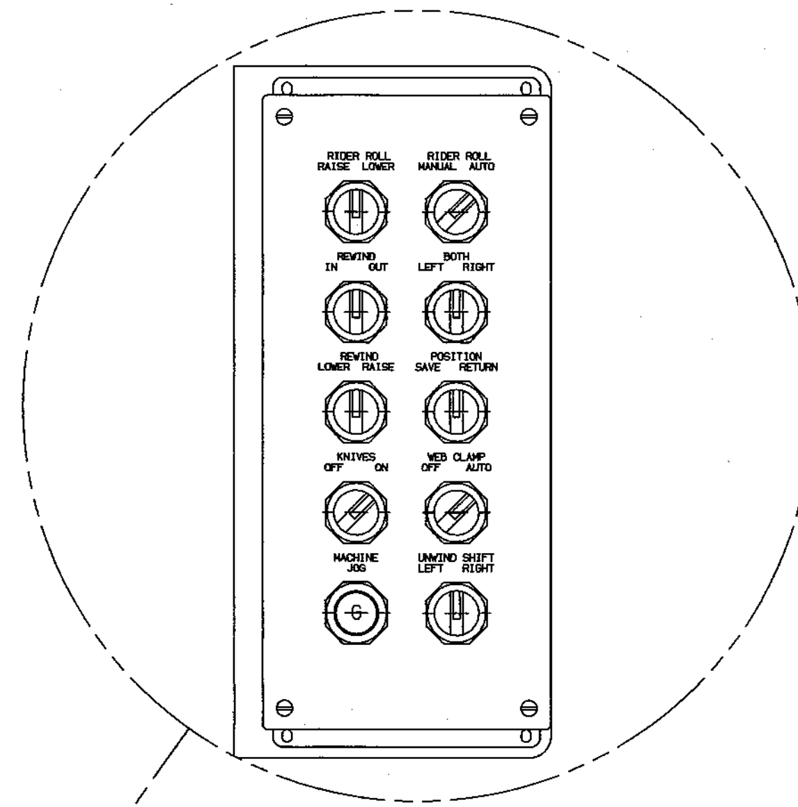
MAIN REWIND CONTROL STATION (RH SIDE)
