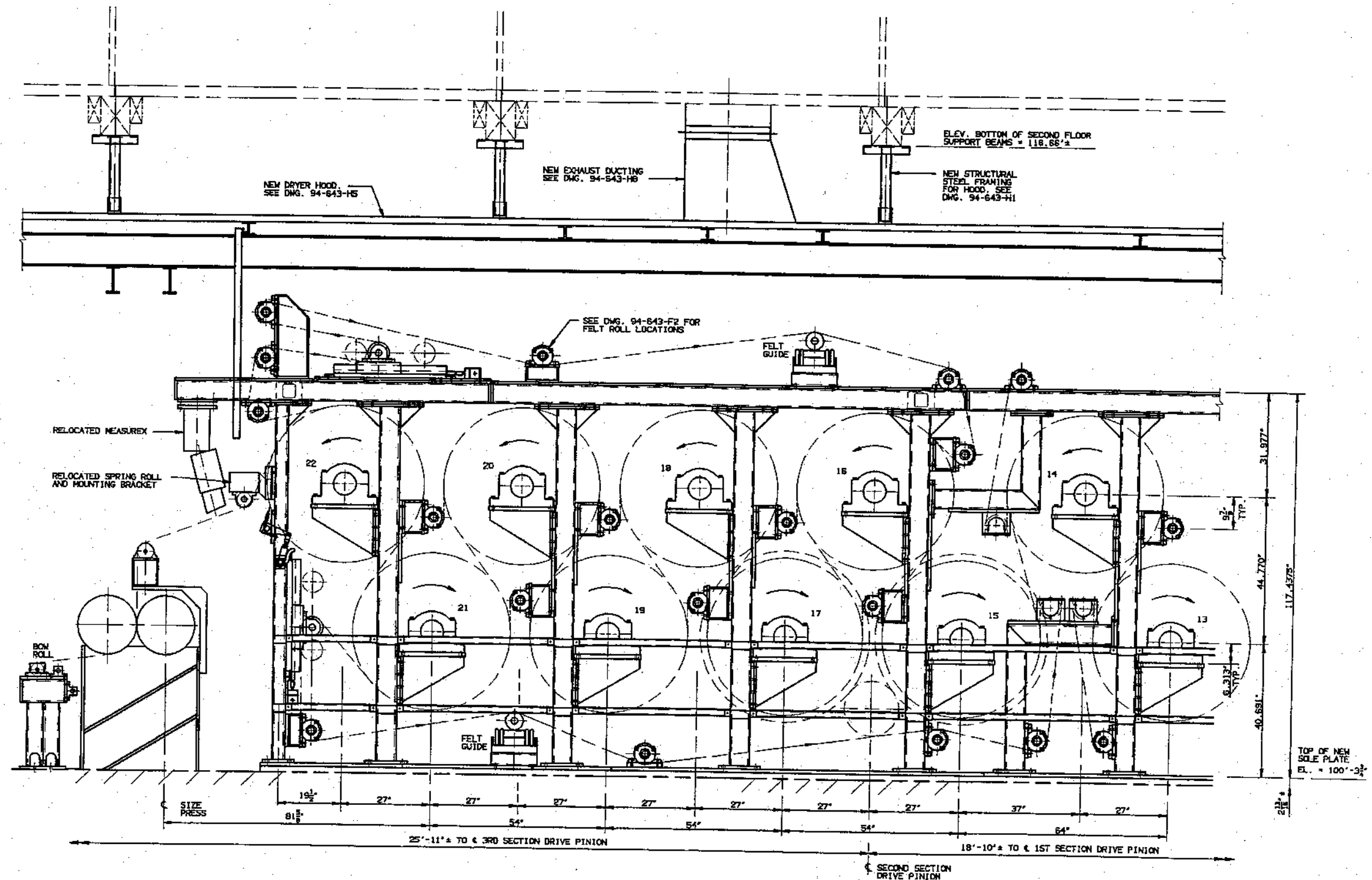
SECOND DRYER SECTION - PROPOSED T.S. ELEVATION
