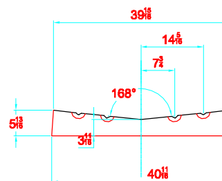
TRANSVERSAL SECTION "A" SECCION TRANSVERSAL "A"
