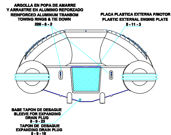
AFT VIEW VISTA TRASERA
