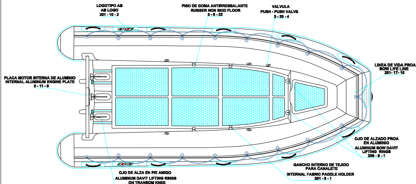
PLANT VIEW VISTA SUPERIOR
