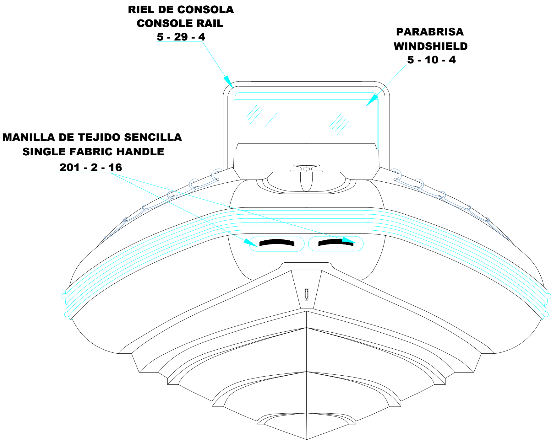
FORE VIEW VISTA FRONTAL
