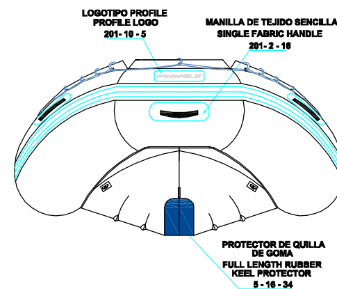
FORE VIEW VISTA FRONTAL
