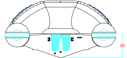
AFT VIEW VISTA TRASERA
