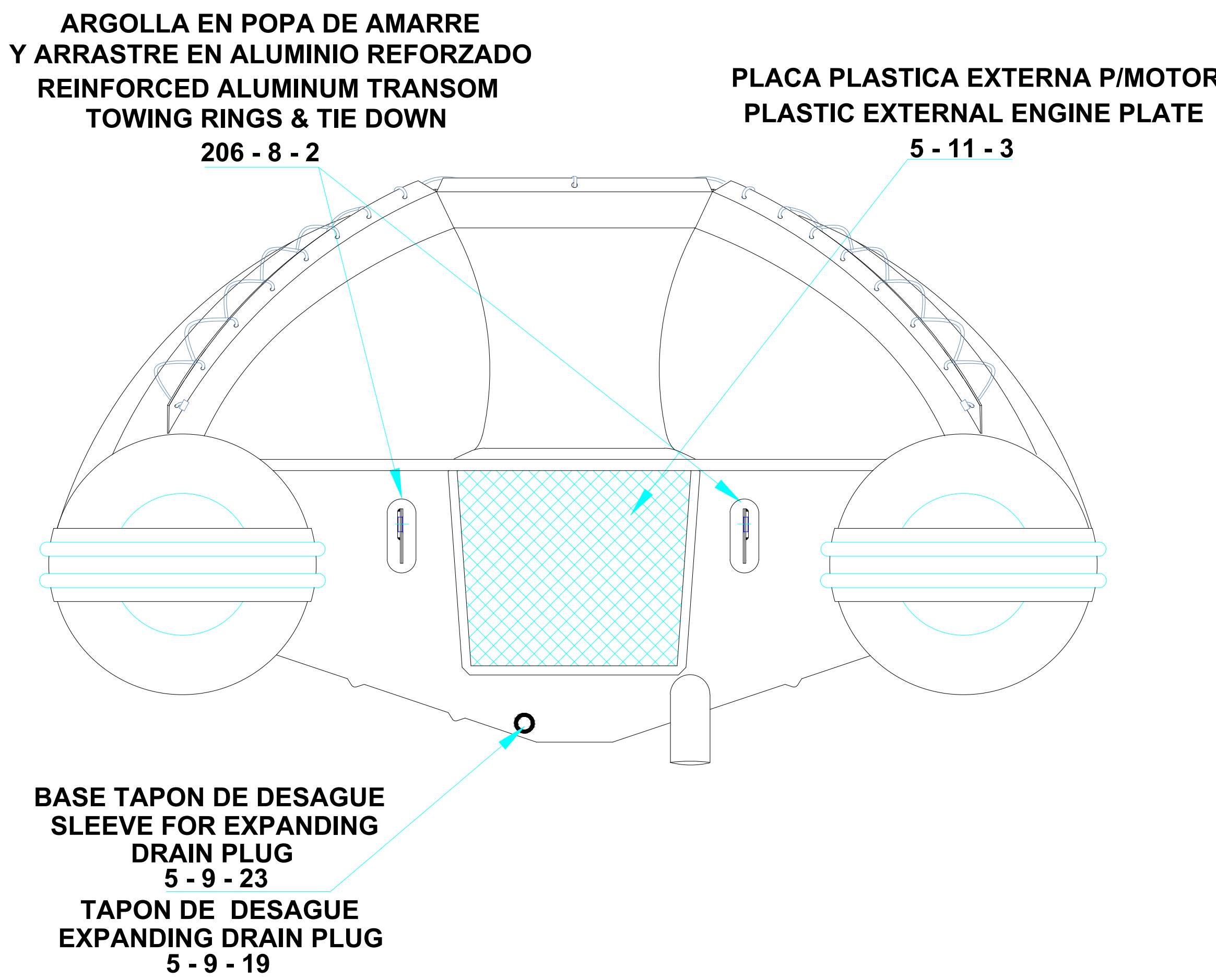
AFT VIEW VISTA TRASERA
