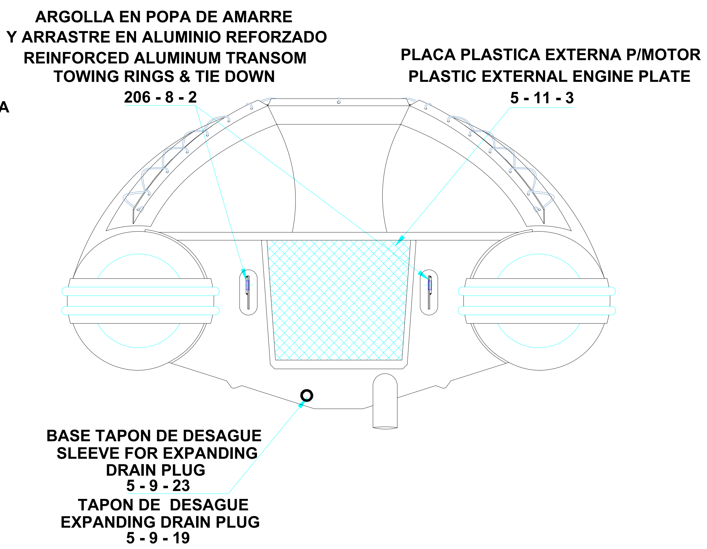
AFT VIEW VISTA TRASERA
