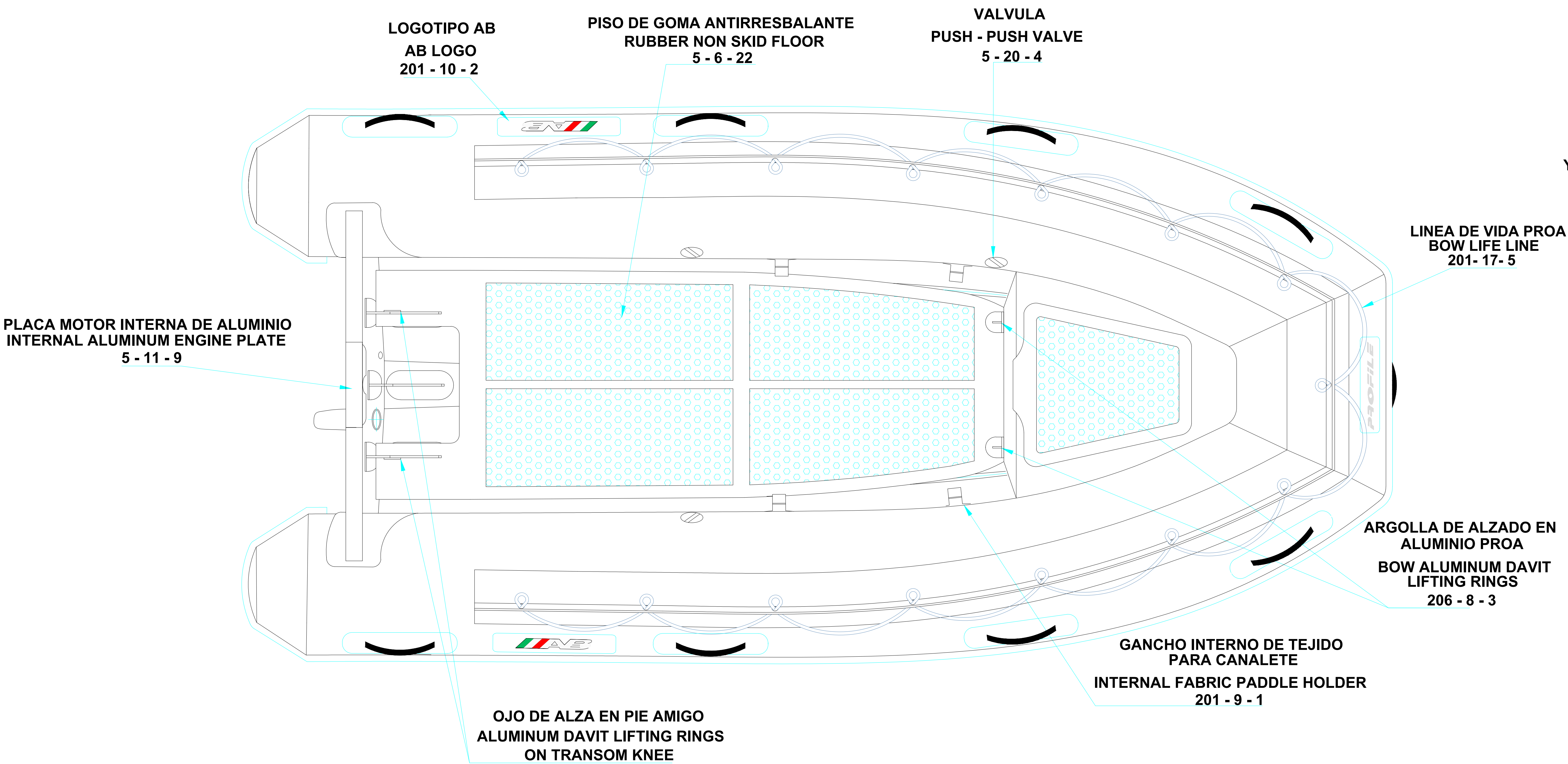
PLANT VIEW VISTA SUPERIOR
