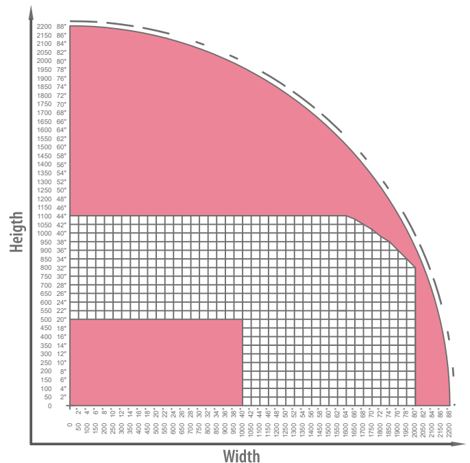
2200 SERIES ROLLER CONVEYOR
