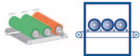
UniSander 2.2.3. 0-5° Surface sanding – more aggressive. High line speed.
