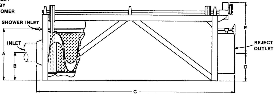
SIDE VIEW
