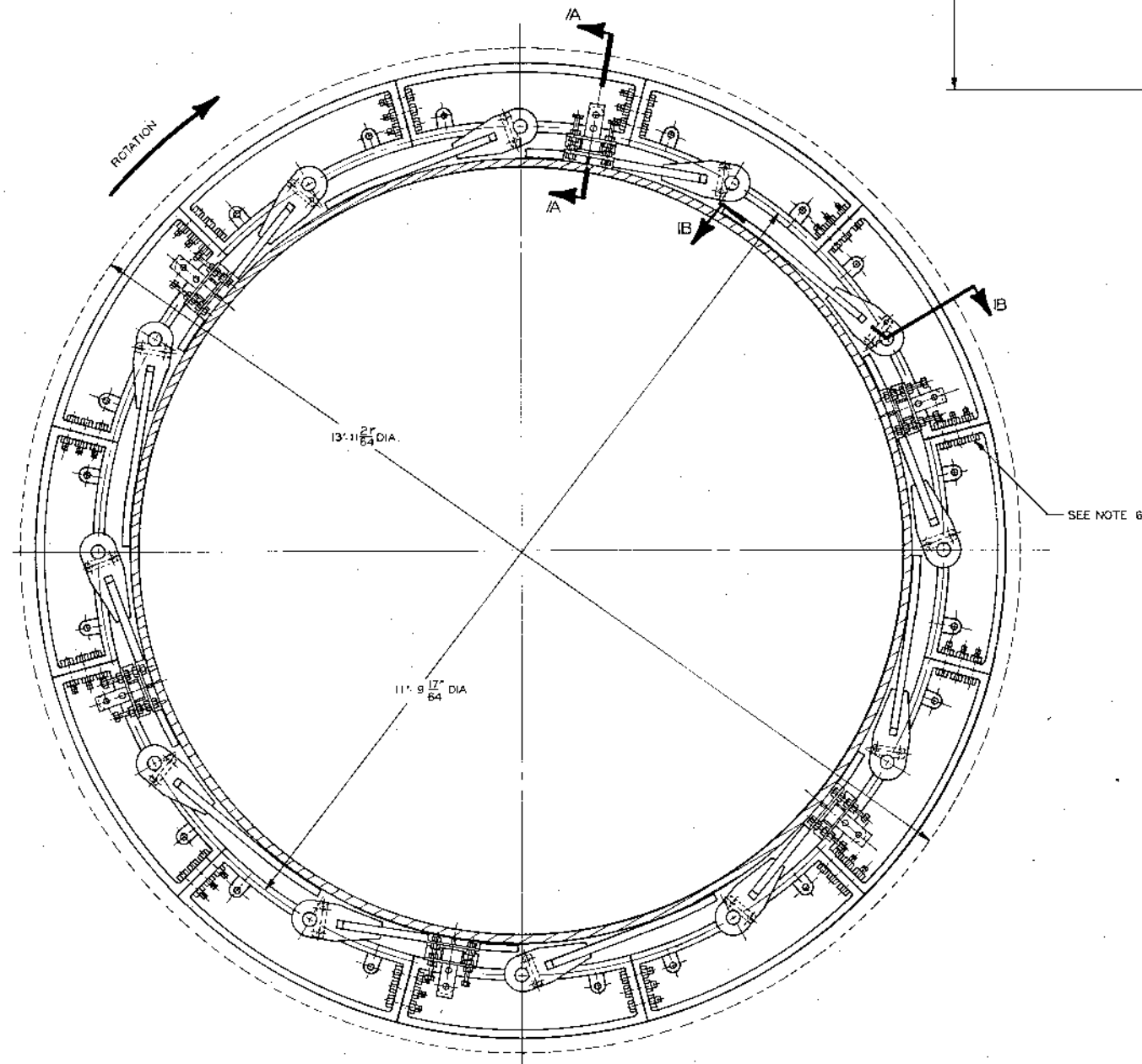
VIEW LOOKING FROM INLET END SCALE: 3/4" = 1'-0"
