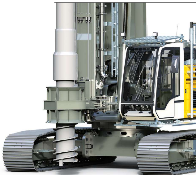
Full displacement tool with auger guide
