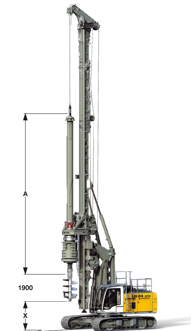
LB 24-270 with optional equipment and automatic casing driver
