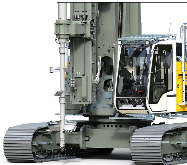
Soil mixing
