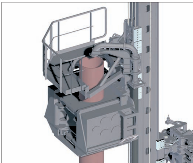
Ring vibrator with platform and concreting system
