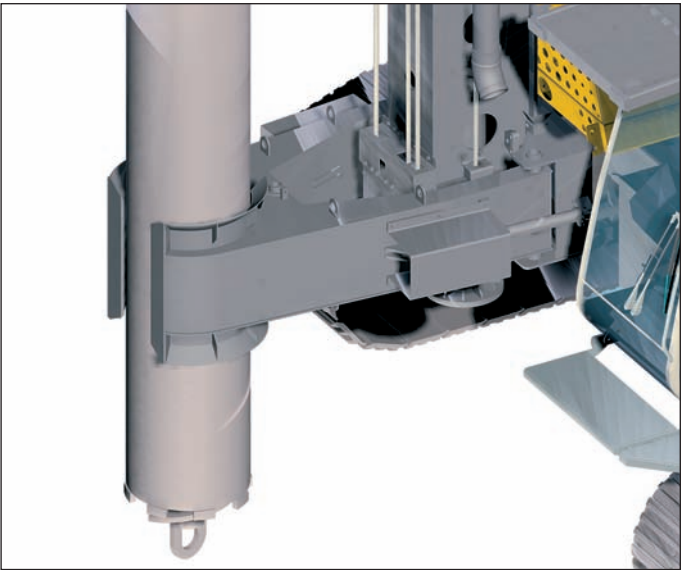
Hydraulic casing guide
