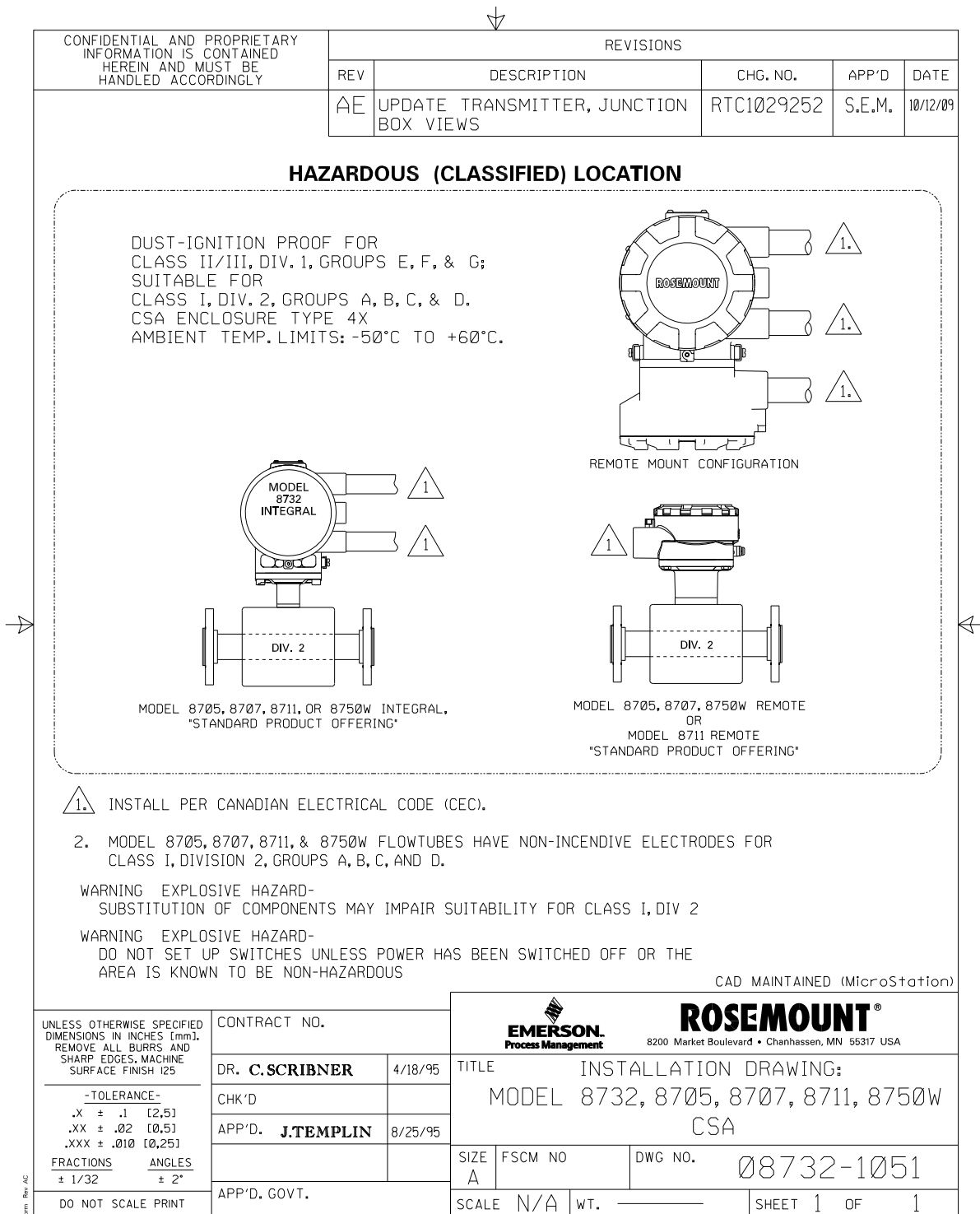
Figure B-15. Installation Drawings Hazardous (Classified Location)
