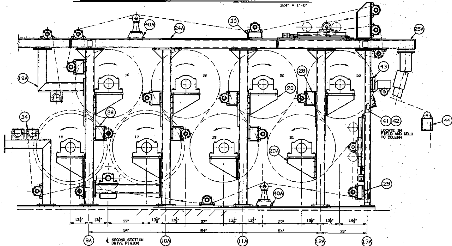
SECOND DRYER SECTION - D.S. DRYER FRAME ASSEMBLY
