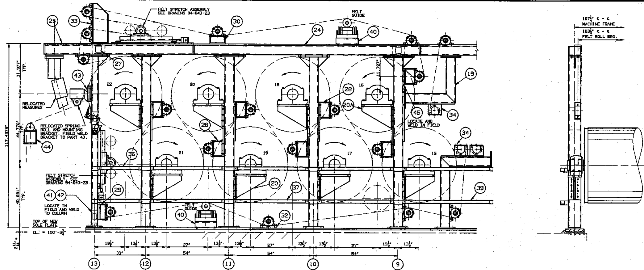
SECOND DRYER SECTION - T.S. DRYER FRAME ASSEMBLY
