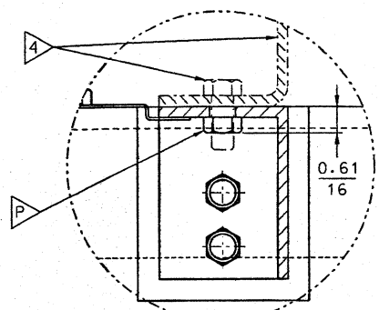
DETAIL B SCALE 1:2 TYP. CHUTE MOUNTING
