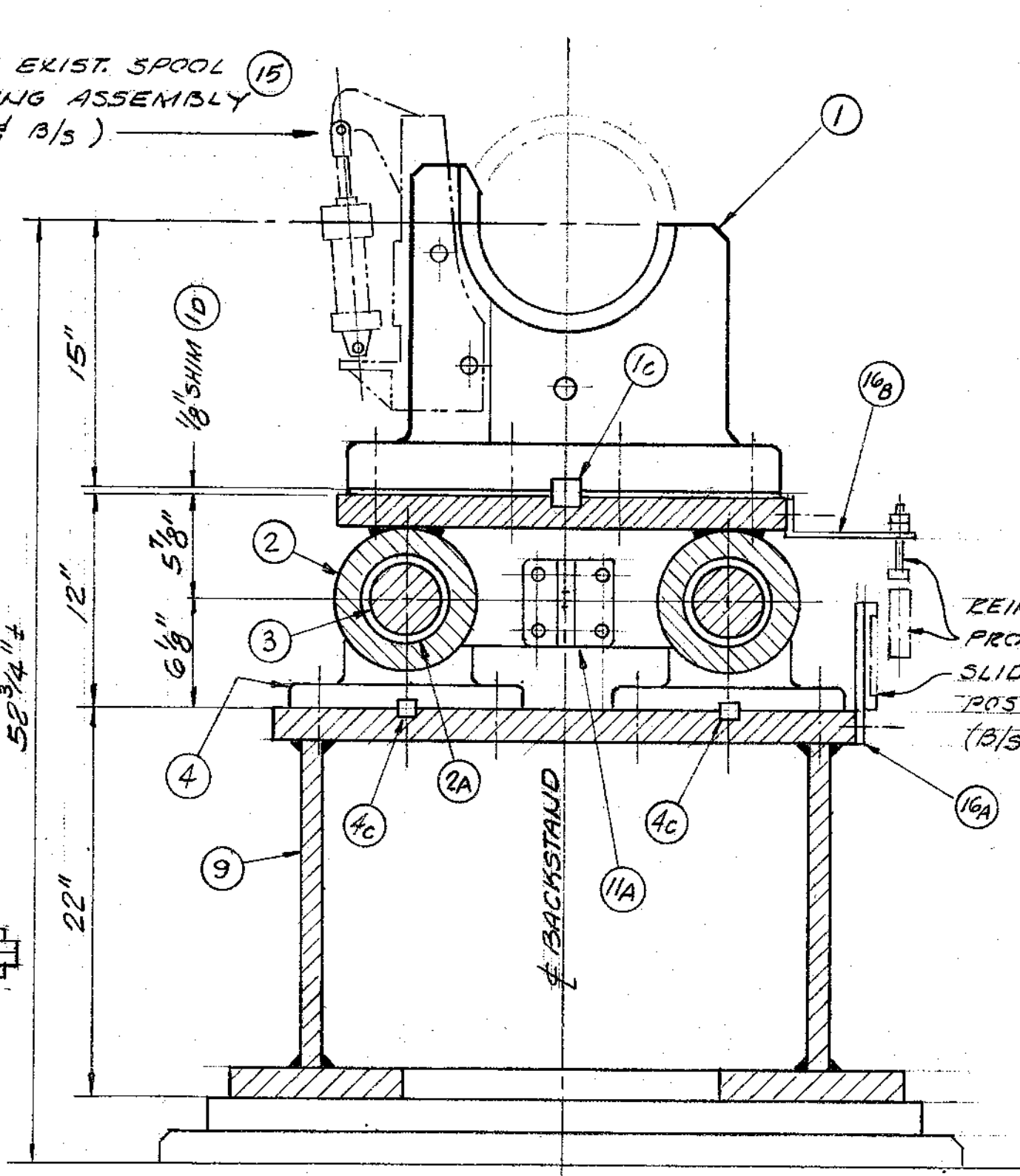
SECTION "C-C" B/3 SHOWN ~ F/3 SIMILAR
