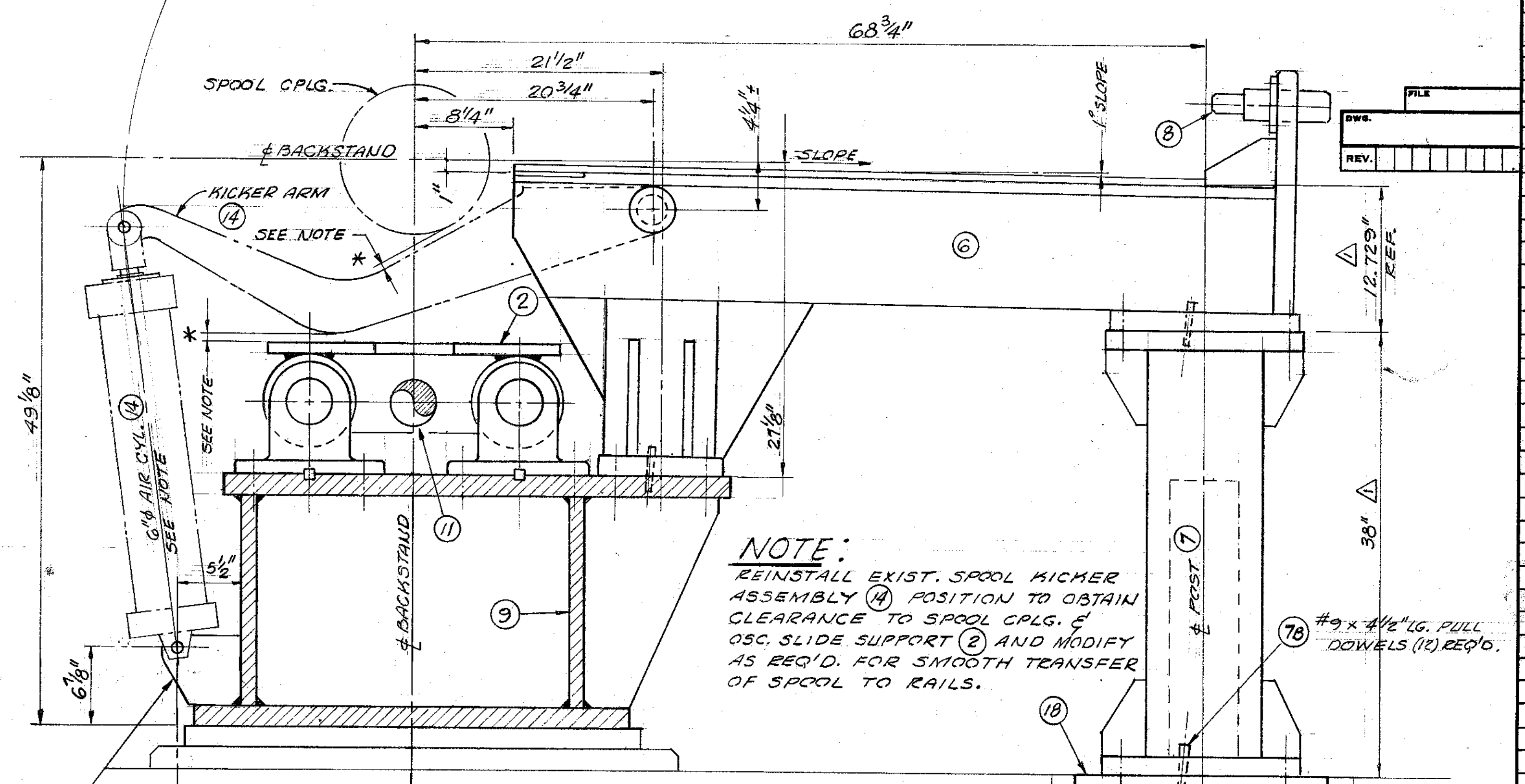
SECTION "B-B" B/3 SHOWN ~ F/3 SIMILAR
