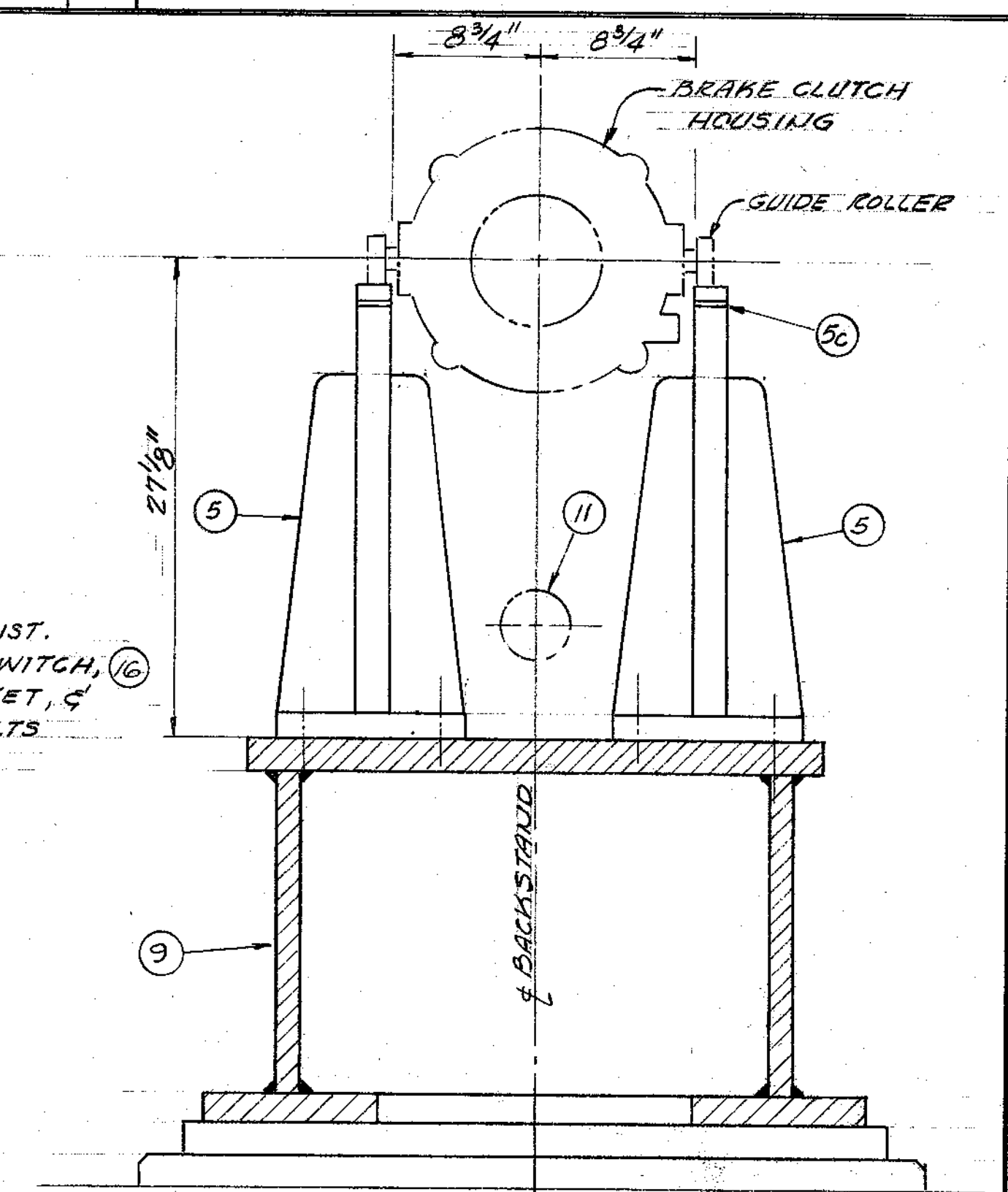
SECTION "A-A"
