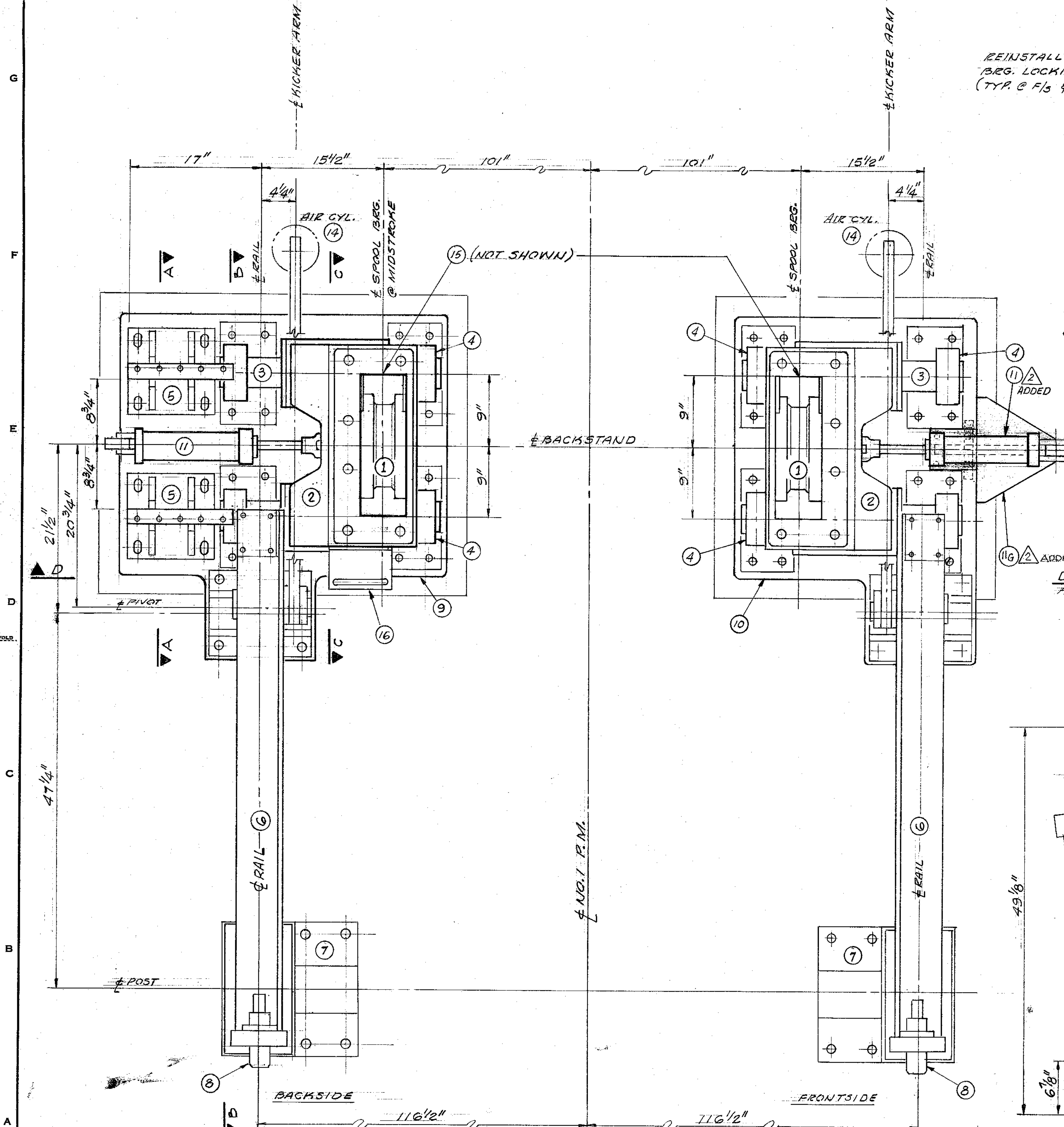
PLAN 1 1/2" = 1'-0"
