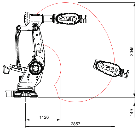
Working range IRB 7710-400/2.85 LID
