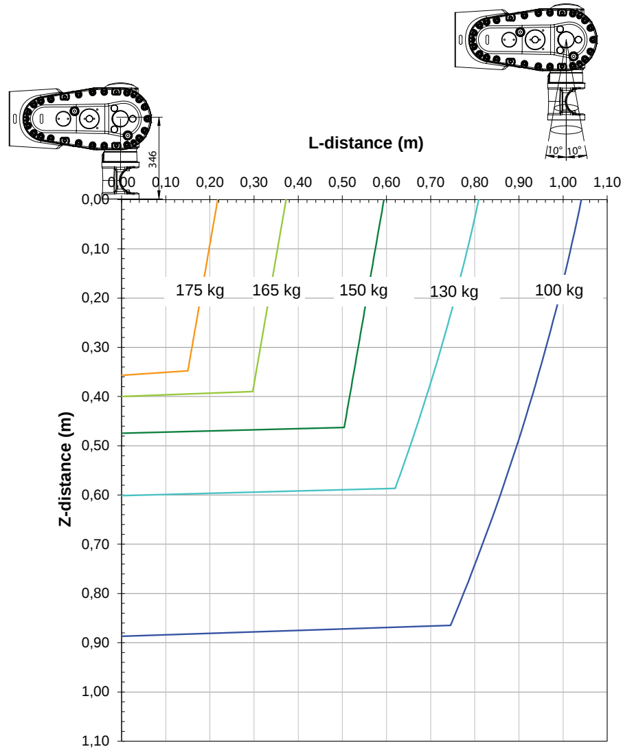
Diagrams of IRB 6720-140/3.2 LID ("Vertical Wrist" ( \pm 10^\circ )) With option [3326-x]. Arm load:LeanID SW.
