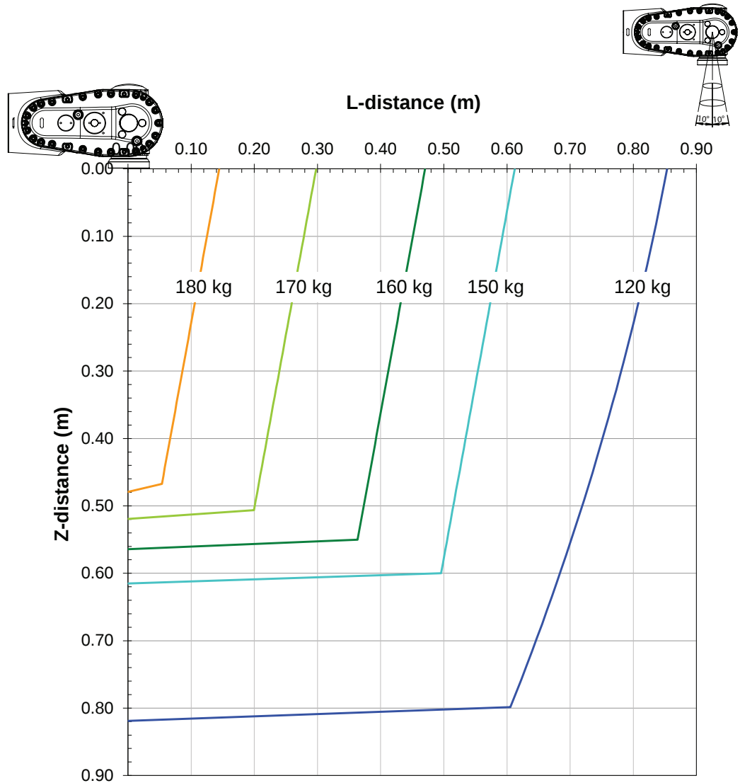
Diagrams of IRB 6720-160/3.2 ("Vertical Wrist" ( \pm 10^\circ )) Arm load for upper arm: 50 kg.
