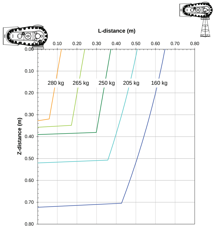
Diagrams of IRB 6720-240/2.65"Vertical Wrist" ( \pm 10^\circ ) Arm load for upper arm: 50 kg.
