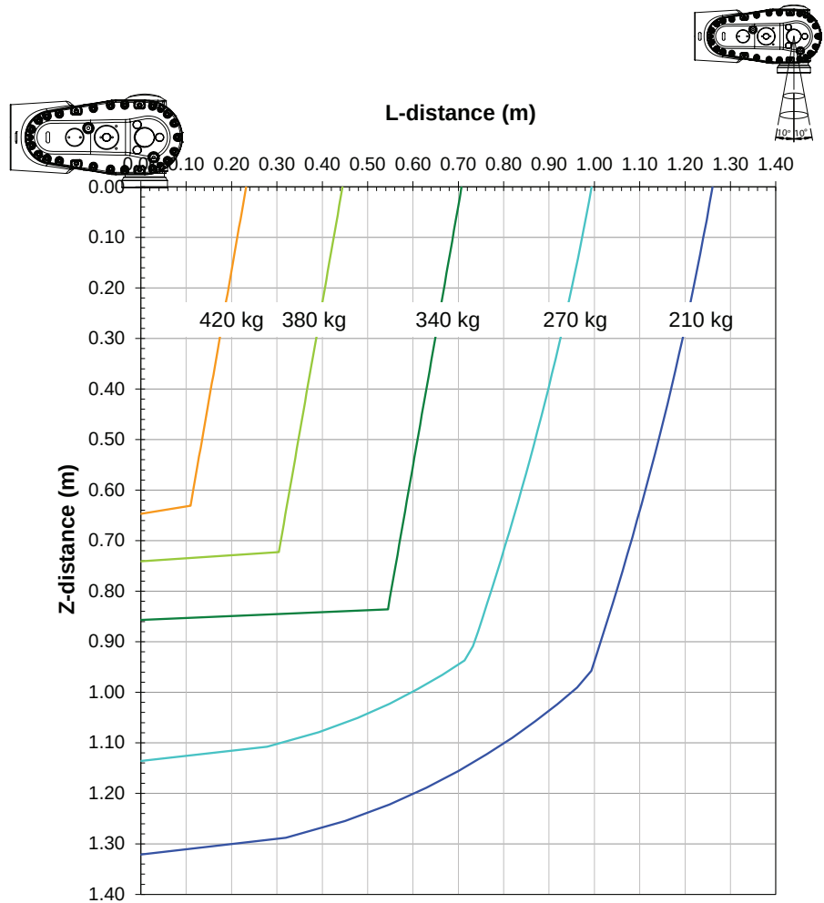
Diagrams of IRB 7710-360/3.3 ("Vertical Wrist" ( \pm 10^\circ )) Arm load for upper arm: 50 kg.
