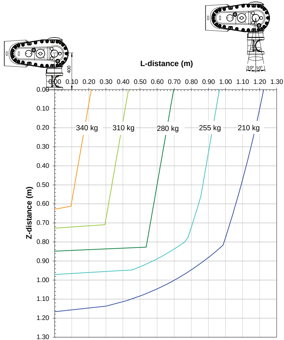
Diagrams of IRB 7710-280/3.5 LID ("Vertical Wrist" ( \pm 10^\circ )) With option [3326-x]. Arm load: LeanID SW.
