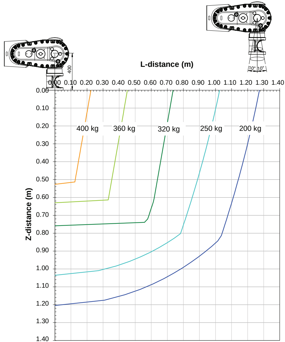
Diagrams of IRB 7710-325/3.3 LID ("Vertical Wrist" ( \pm 10^\circ )) With option [3326-x]. Arm load: LeanID SW.
