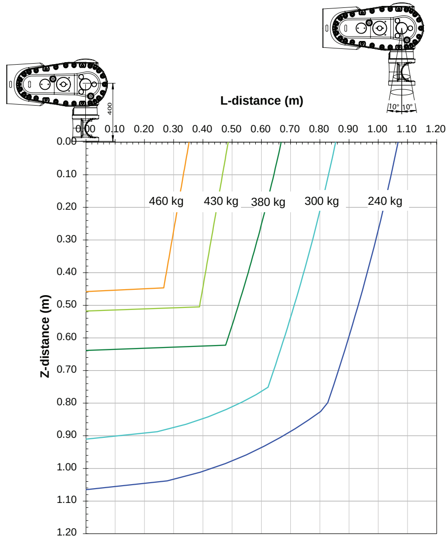
Diagrams of IRB 7710-390/3.1 LID ("Vertical Wrist" ( \pm 10^\circ )) With option [3326-x]. Arm load: LeanID SW.
