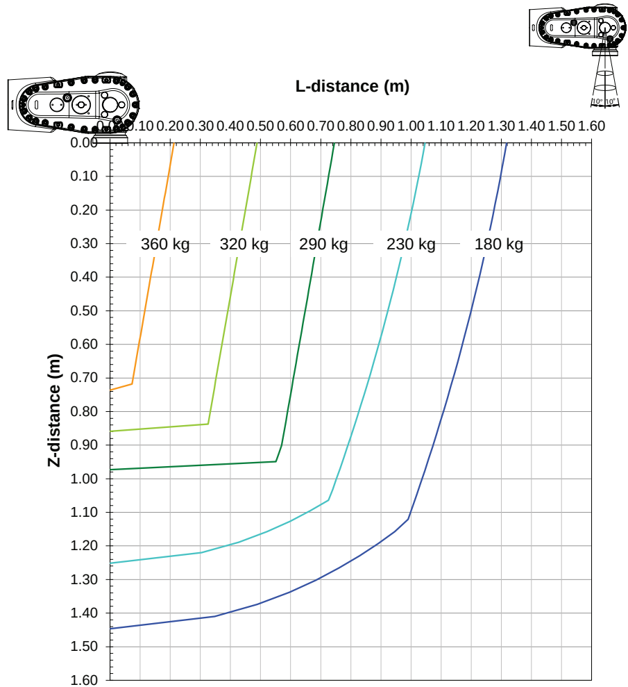
Diagrams of IRB 7710-310/3.5 ("Vertical Wrist" ( \pm 10^\circ )) Arm load for upper arm: 50 kg.
