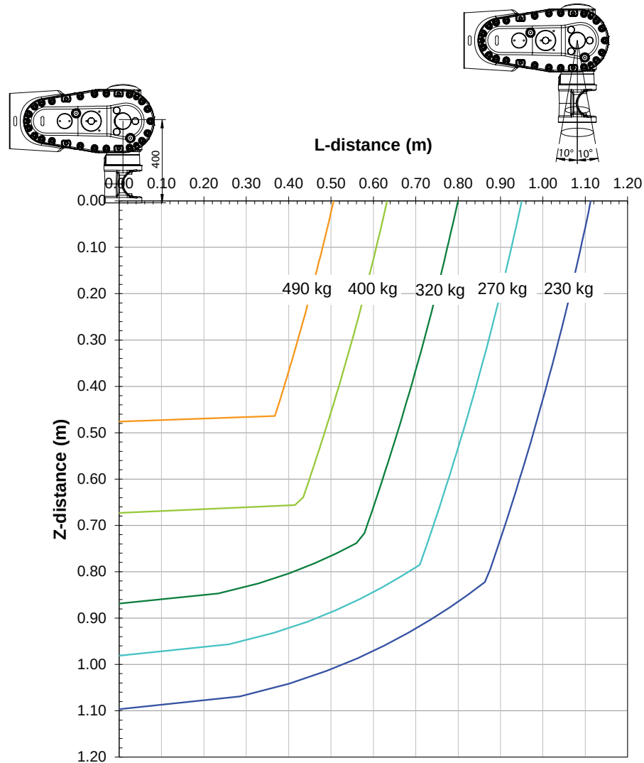
Diagrams of IRB 7710-400/2.85 LID ("Vertical Wrist" ( \pm 10^\circ )) With option [3326-x]. Arm load: LeanID SW.
