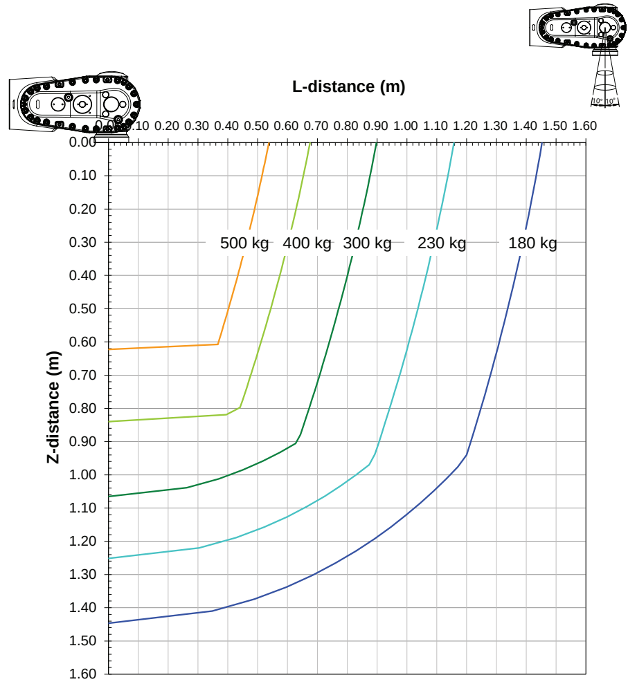
Diagrams of IRB 7710-500/2.85"Vertical Wrist" ( \pm 10^\circ ) Arm load for upper arm: 50 kg.
