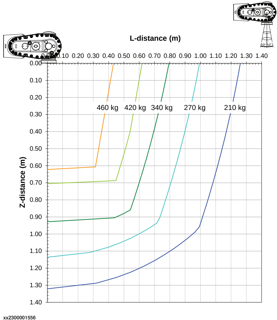
Diagrams of IRB 7710-430/3.1"Vertical Wrist" ( \pm 10^\circ ) Arm load for upper arm: 50 kg.
