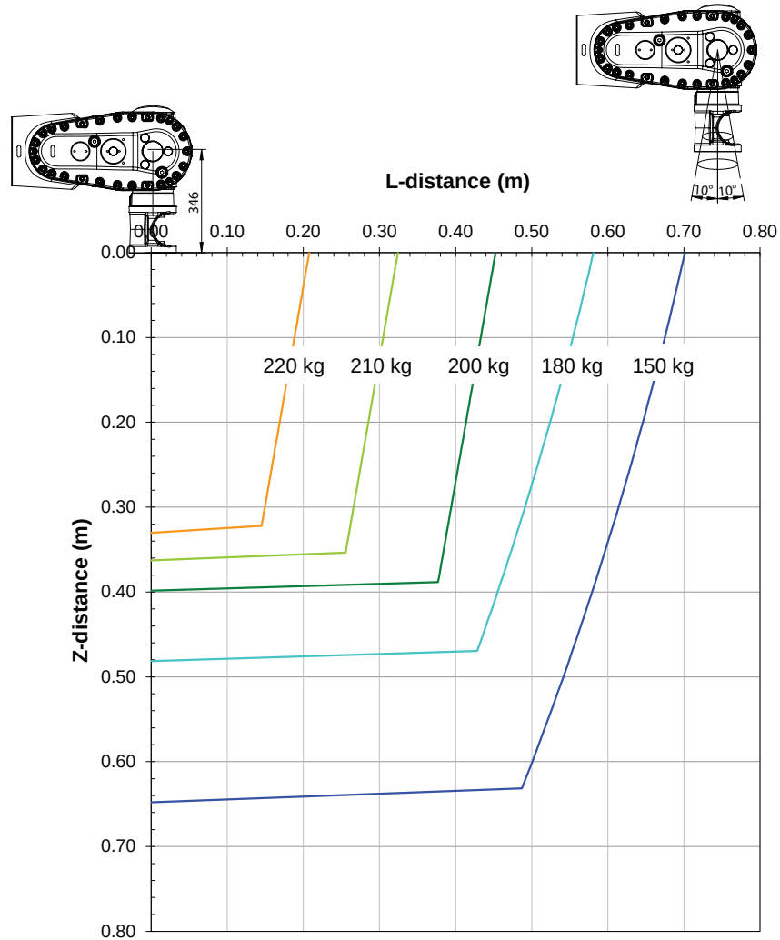
Diagrams of IRB 6730-190/3.1 LID ("Vertical Wrist" ( \pm 10^\circ )) With option [3326-x]. Arm load: LeanID SW.
