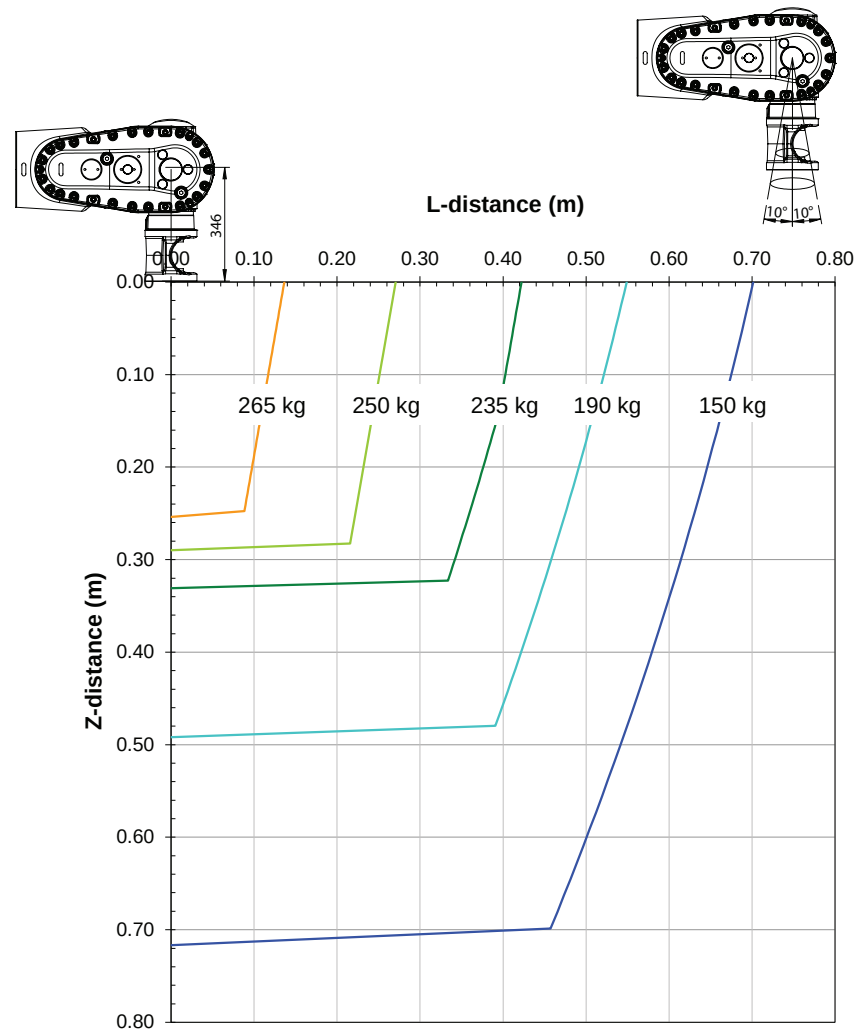
Diagrams of IRB 6730-220/2.9 LID ("Vertical Wrist" ( \pm 10^\circ )) With option [3326-x]. Arm load: LeanID SW.
