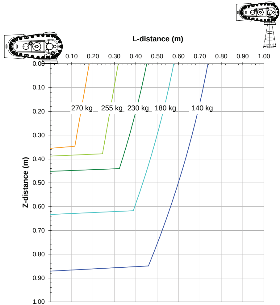
Diagrams of IRB 6730-240/2.9"Vertical Wrist" ( \pm 10^\circ ) Arm load for upper arm: 50 kg.
