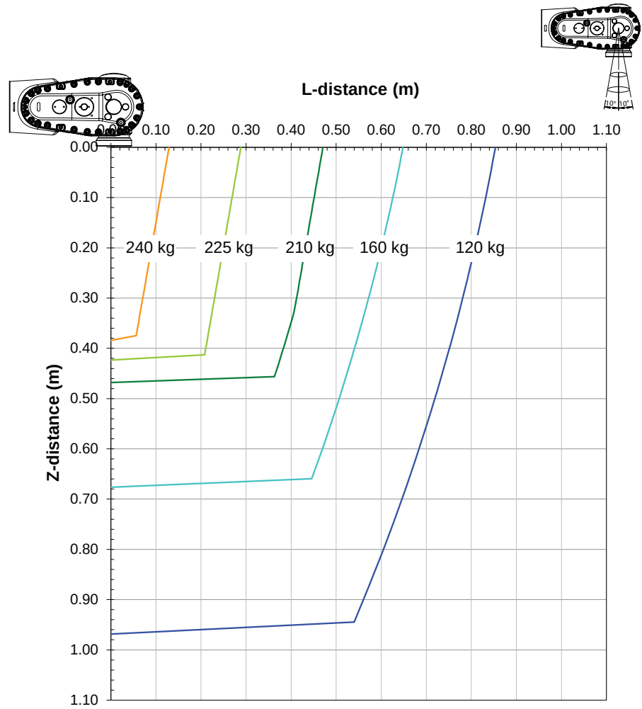
Diagrams of IRB 6730-210/3.1 ("Vertical Wrist" ( \pm 10^\circ )) Arm load for upper arm: 50 kg.
