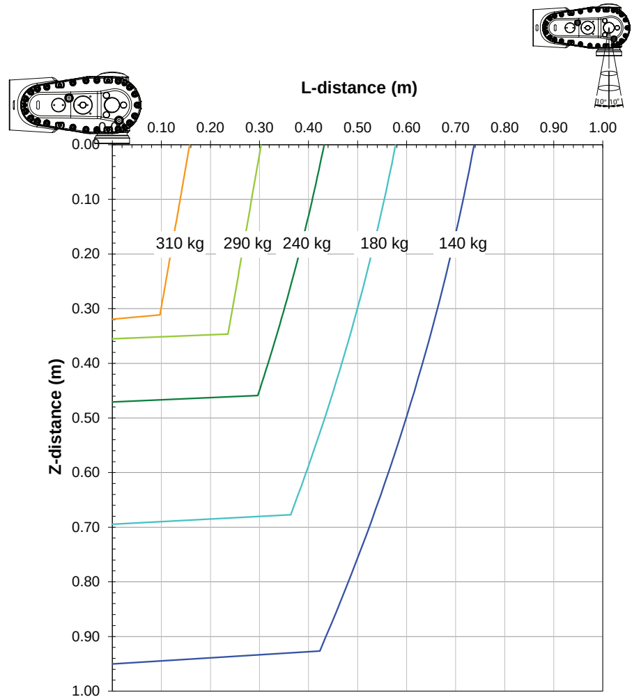
Diagrams of IRB 6730-270/2.7"Vertical Wrist" ( \pm 10^\circ ) Arm load for upper arm: 50 kg.
