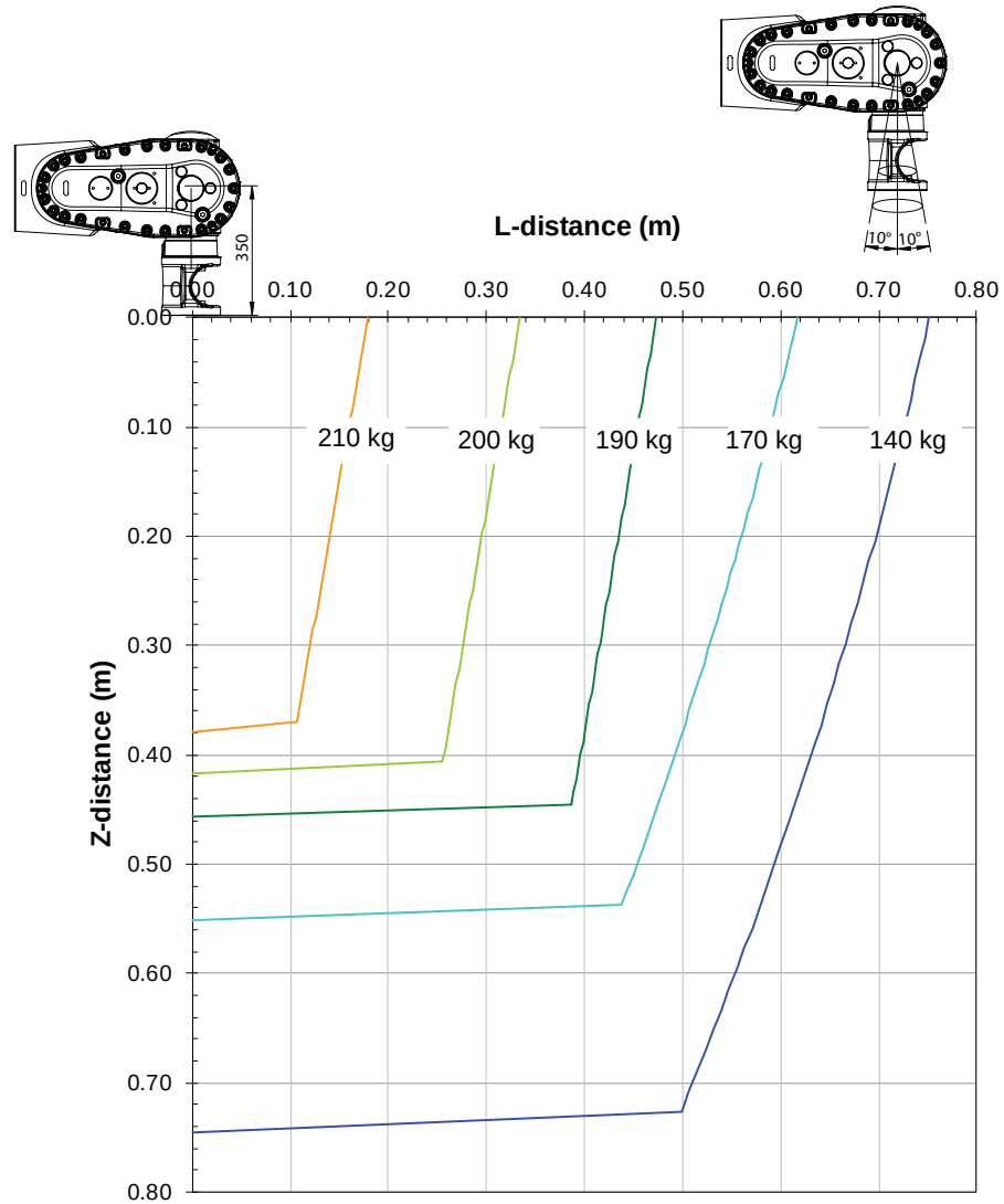
Diagrams of IRB 6730S-180/3.5 LID ("Vertical Wrist" ( \pm 10^\circ )) With option [3326-x]. Arm load: LeanID SW.
