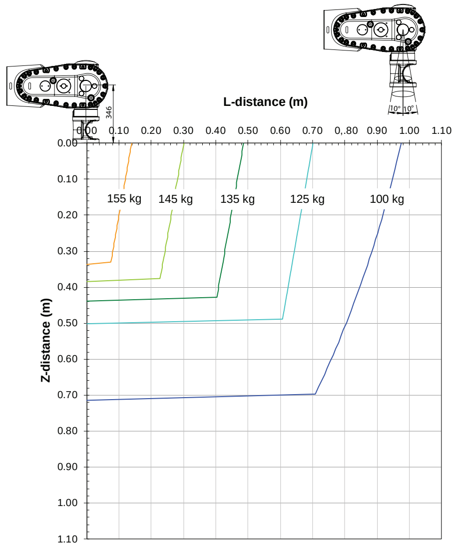
Diagrams of IRB 6730S-130/4.0 LID ("Vertical Wrist" ( \pm 10^\circ )) With option [3326-x]. Arm load: LeanID SW.
