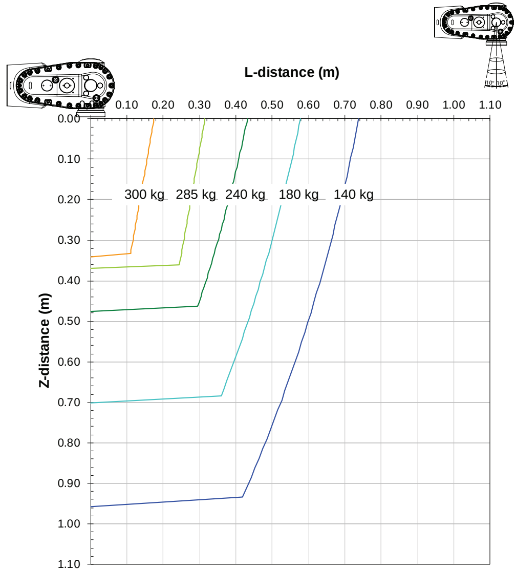
Diagrams of IRB 6730S-270/3.1"Vertical Wrist" ( \pm 10^\circ ) Arm load for upper arm: 50 kg.
