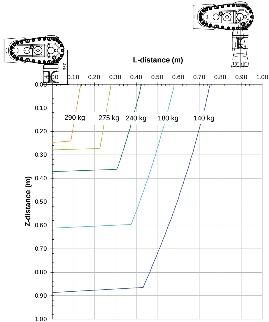
Diagrams of IRB 6730S-220/3.1 LID ("Vertical Wrist" ( \pm 10^\circ )) With option [3326-x]. Arm load: LeanID SW.
