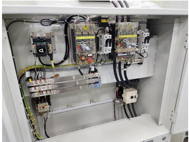
D. Control Unit 3
