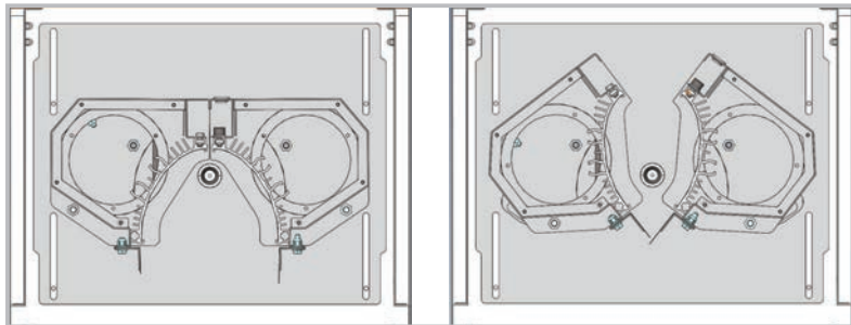
Lamp unit with shutter for stand-by management. High cooling efficiency
