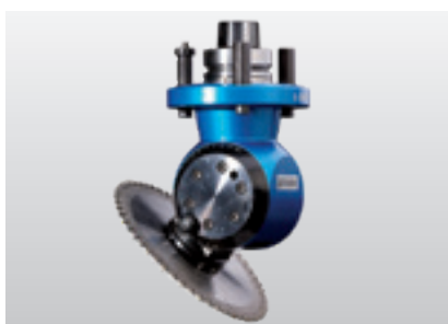
Drilling/Sawing, swivelling* , (0° - 90°)
