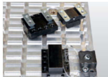
Aluminium matrix table with trapeze shaped grooves for interlocking and flexible fixing of all kinds of clamping aids
