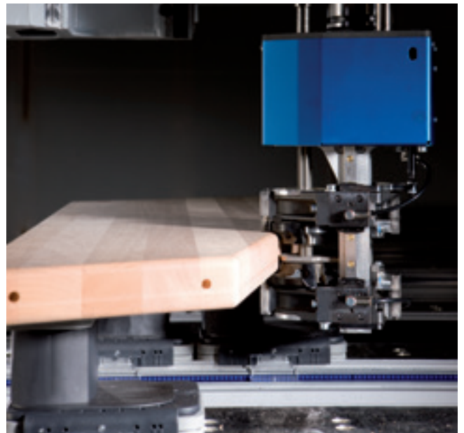
Pneumatic interface – the patented interface with 3-way support on all C-axes and 5-axis heads enables the use of traced units, e.g. for precise rounding off at the top and bottom no matter the thickness tolerances.
