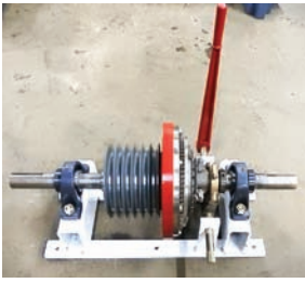
12181 $4,600.00 SUPREME MFG INLINE CLUTCH 11-1/2" dia clutch pads, rated up to 150hp, 2-3/16" dia through shaft, 91/2" dia 6 groove C-belt pulley, BRAND NEW! ready to ship 260-633-4047 Wolcottville, IN
