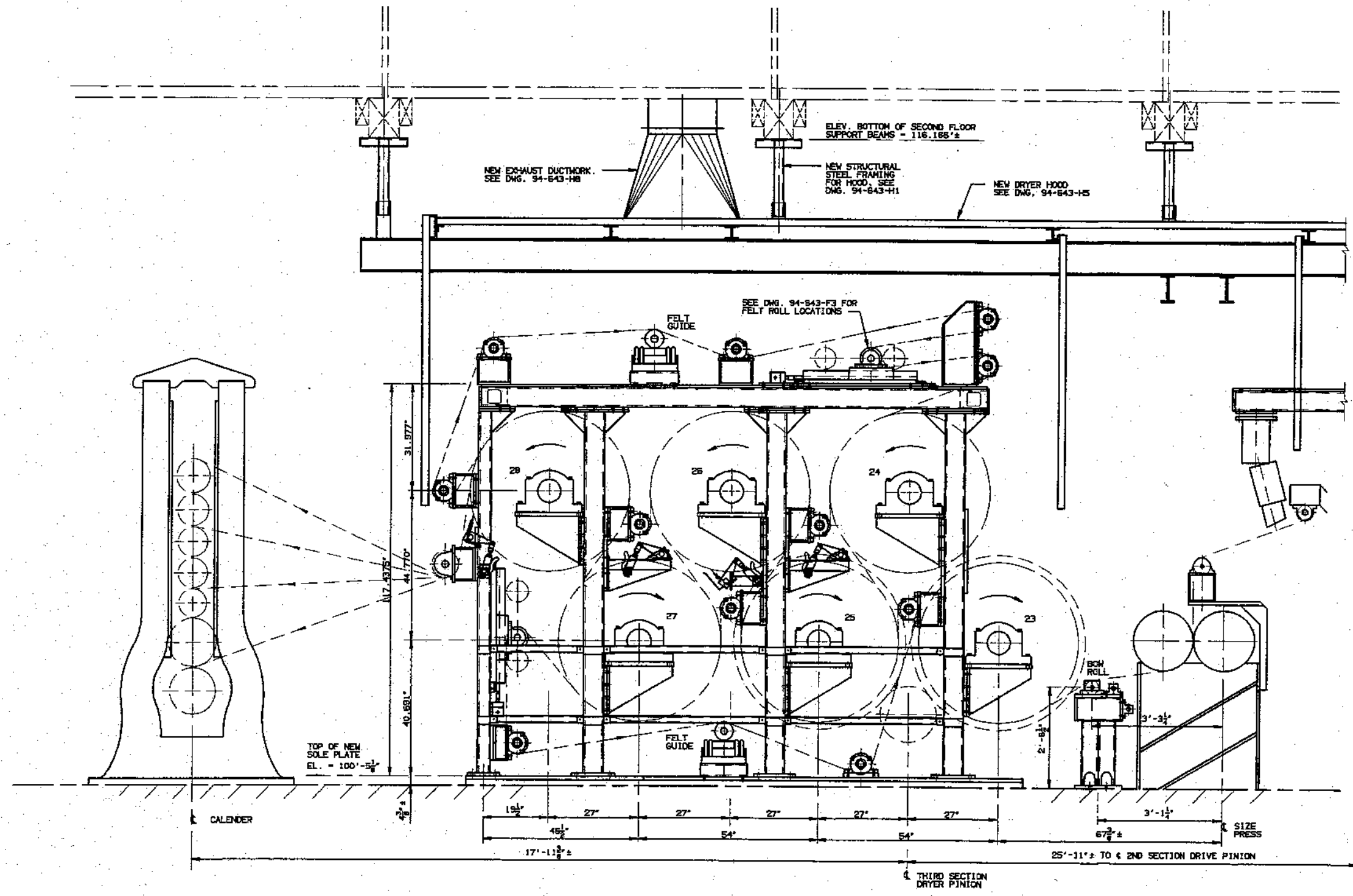
THIRD DRYER SECTION - PROPOSED T.S. ELEVATION 3/4" = 1'-0"
