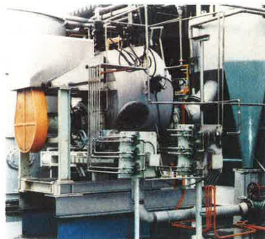
The Helipoire System consists of the Helico High-consistency Pulper (right) and the Poire/Scavenger.
