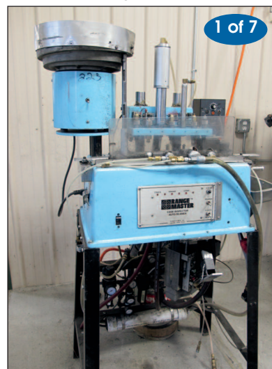
SCHARCH RANGE MASTER CASE INSPECTOR/REAMER
