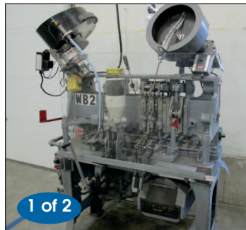
WATERBURY FARREL 7 POSITION 223 CALIBER AMMUNITION LOADER
