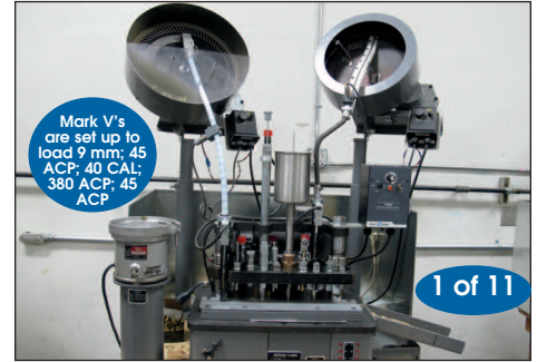
MARK V 9 STATION AMMUNITION LOADER
