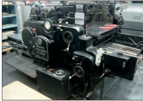
ORIGINAL HEIDELBERG CYLINDER PRESS MODEL SBB, 56X82CM
