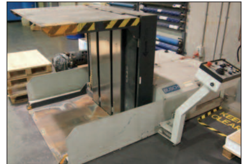
BUSCH PILE TURNER MODEL SWH125RLA
