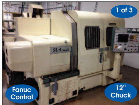
MORI-SEIKI # SL-4 CNC Lathe
