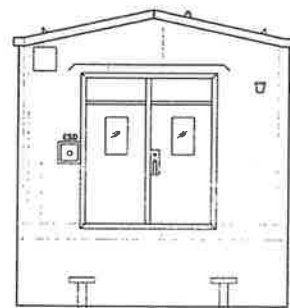
SOUTH EXTERIOR ELEVATION
