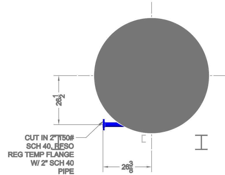
SECTION C-C
