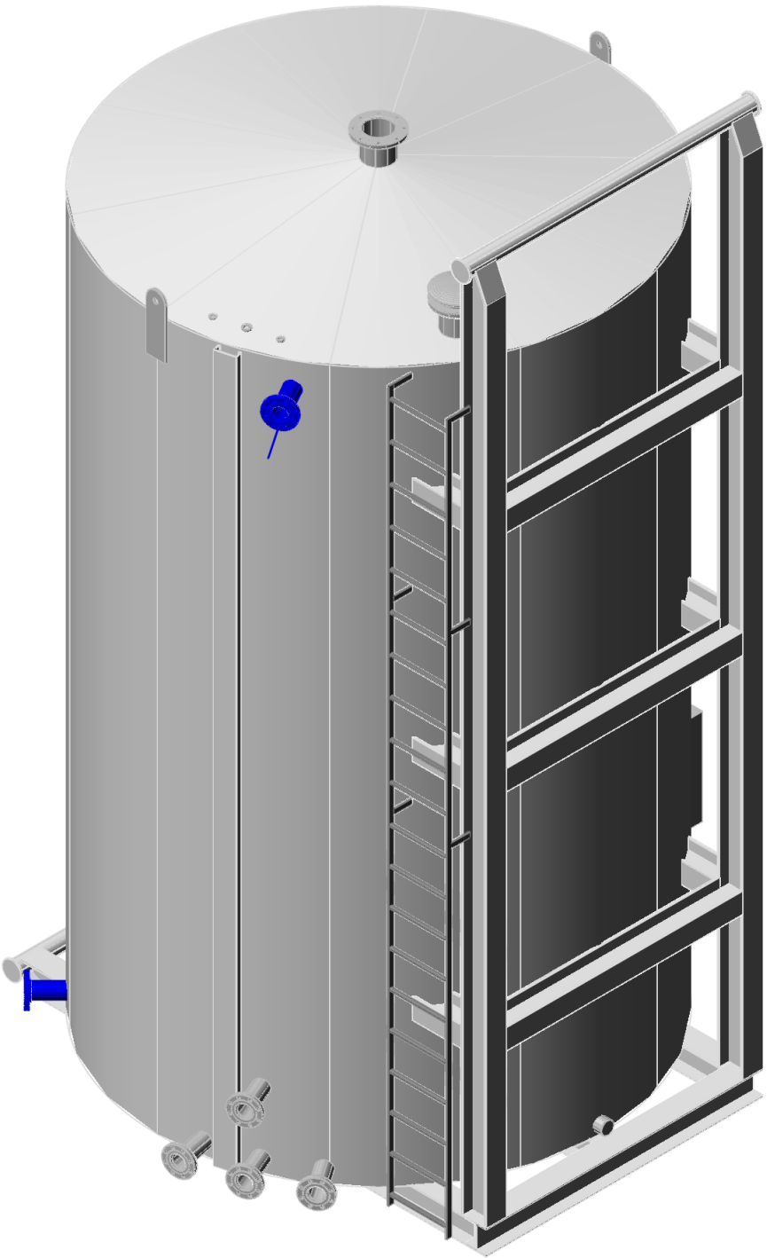
SW ISOMETRIC
