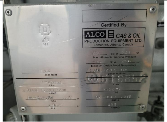
Nameplate
