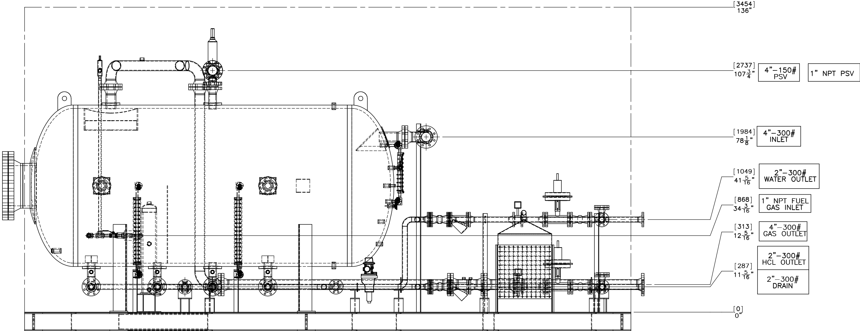
ELEVATION VIEW
