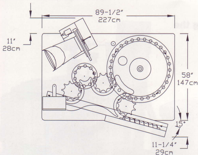
Left Hand with Rotary Cap Feeder
