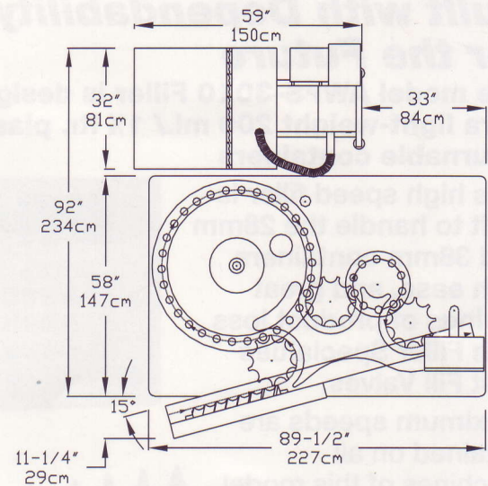
Right Hand with FS 12 Cap Feeder
