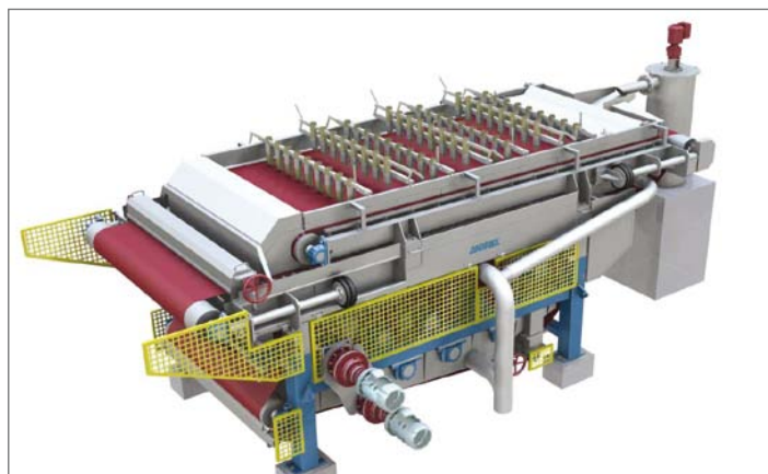
▲ CPF Rhino (with pre-dewatering gravity zone) for dewatering of sludges with up to 100% biological content
