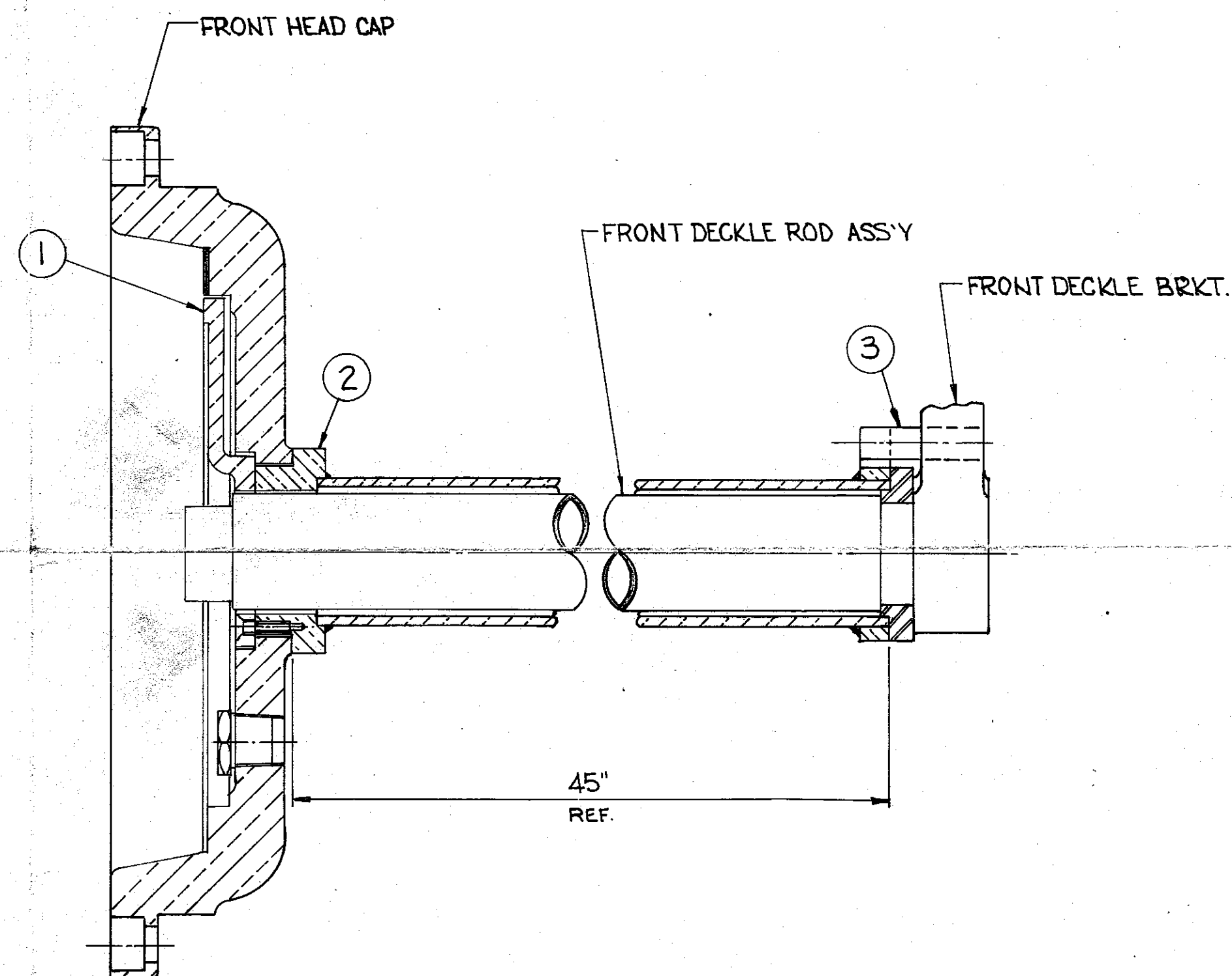
SECTION "A-A"
