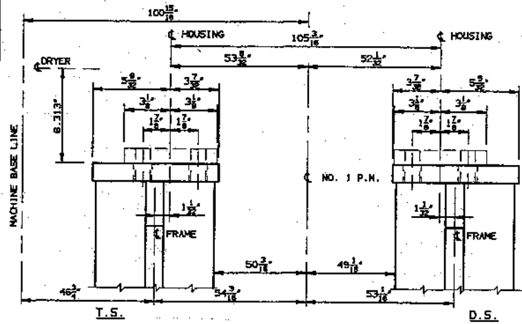
TYP. DETAIL AT DRYER BEARING 3" = 1'-0"
