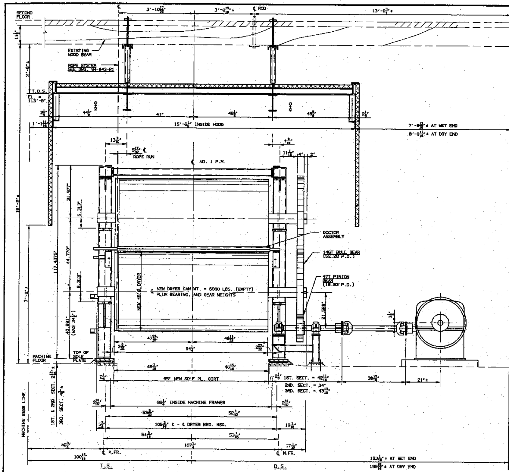
PROPOSED MACHINE CROSS SECTION THRU DRYER CANS 3/4" = 1'-0"
