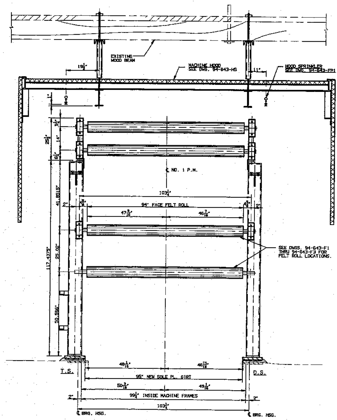
PROPOSED MACHINE CROSS SECTION THRU FELT ROLLS 3/4" = 1'-0"
