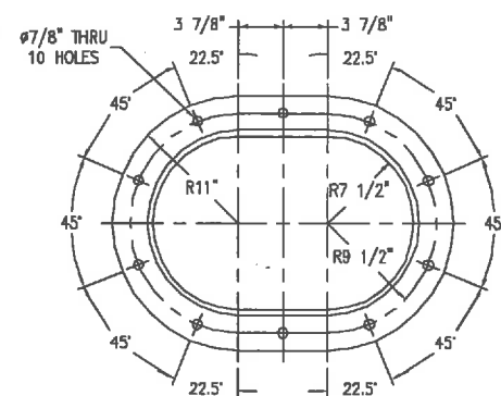
VIEW B-B (INLET FLANGE) SCALE: 1/8"=1"
