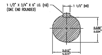
SECT. B-B TYP. SCALE: 3"-1'-0"
